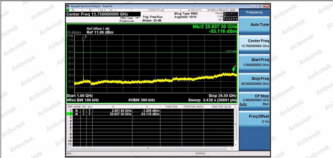
BLE_1M-Ant1-2402-1000~26500-PASS
