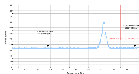
802.11n HT20-Channel 144: Peak
