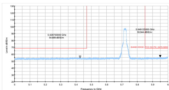
802.11a-Channel 144: Peak
