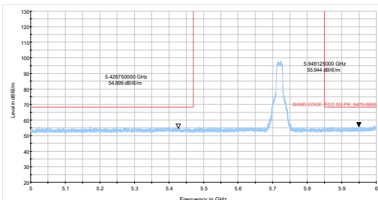
802.11a-Channel 144: Peak
