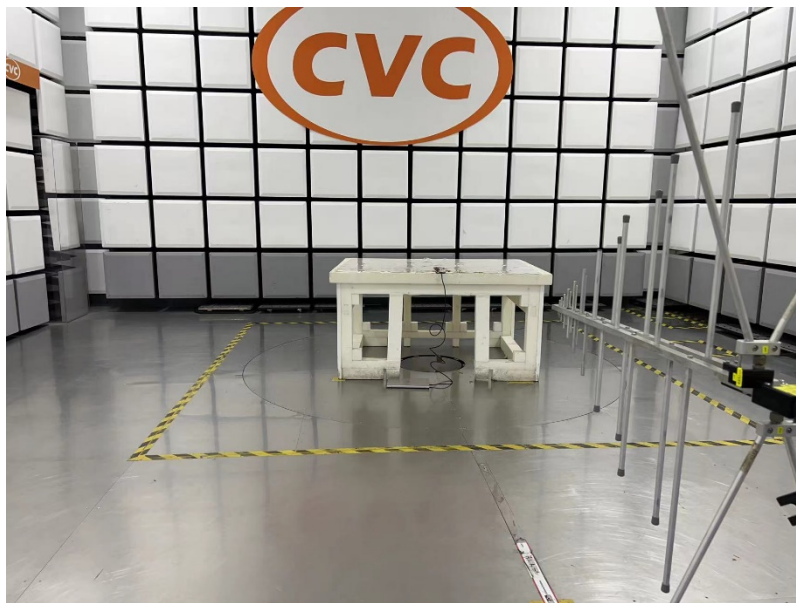
(2) Radiated spurious emission Test Setup(Below 1GHz)
