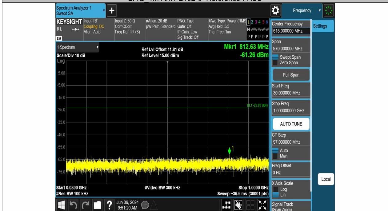
2.4G_1M-Ant1-2402-30~1000-PASS
