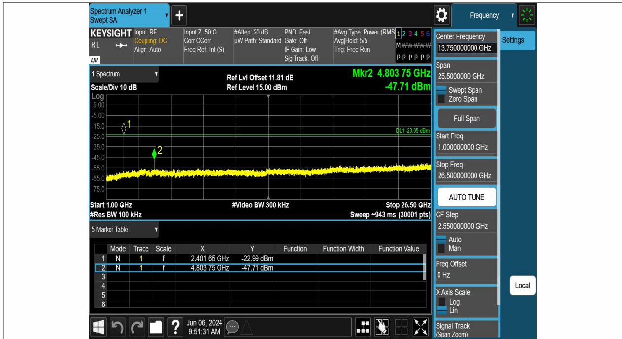
2.4G_1M-Ant1-2402-1000~26500-PASS
