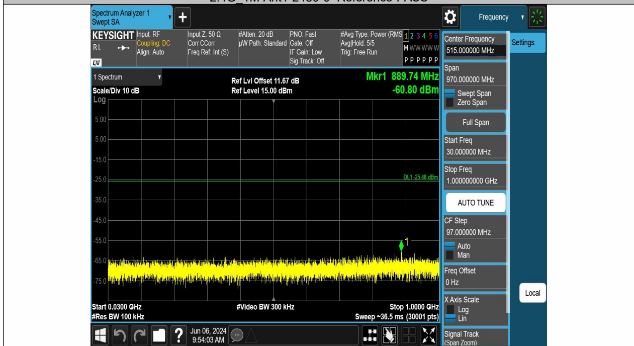
2.4G_1M-Ant1-2480-30~1000-PASS
