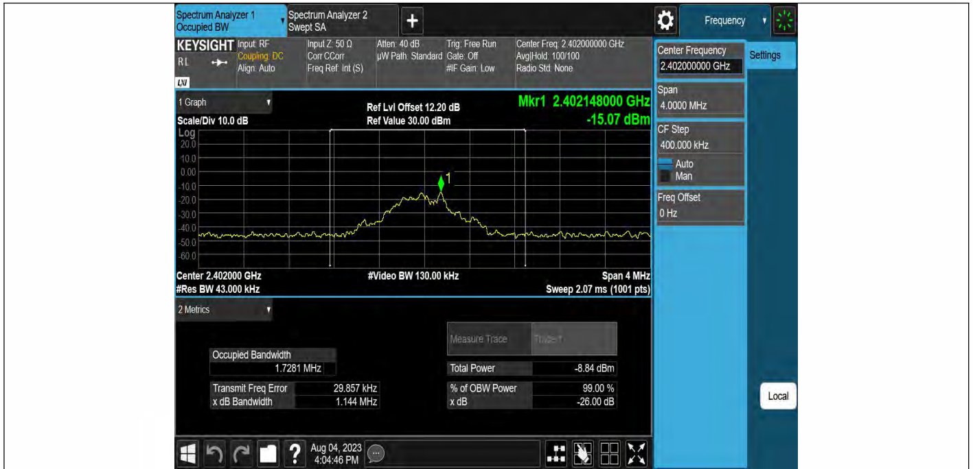
GFSK_1M-Ant1-2402
