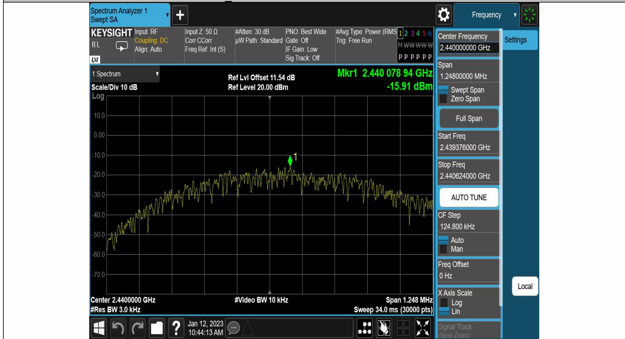
BLE_1M-Ant1-2440--15.92-0.00-0.00-0.00
