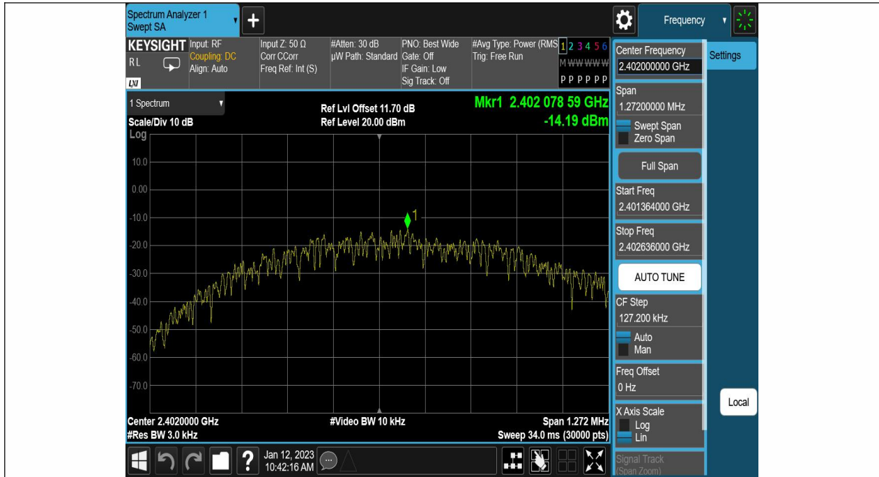
BLE_1M-Ant1-2402--14.19-0.00-0.00-0.00
