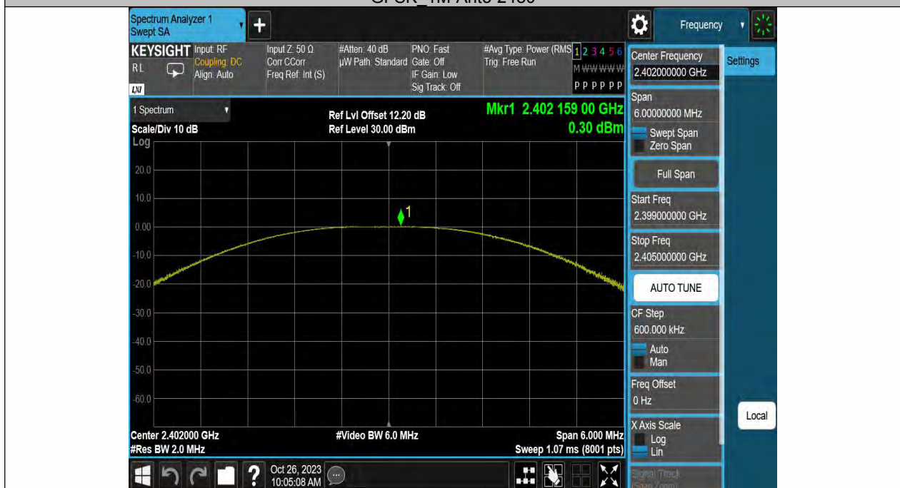
GFSK 2M-Ant3-2402
