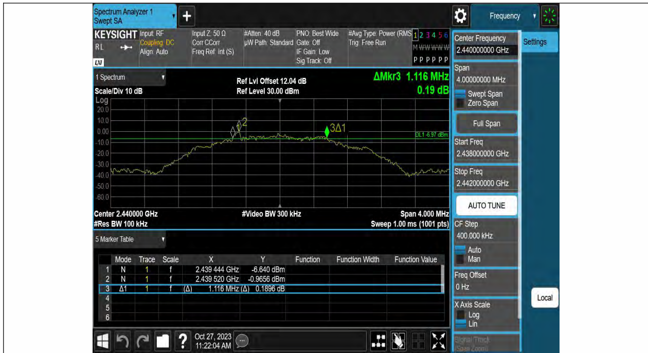
GFSK_2M-Ant1-2440
