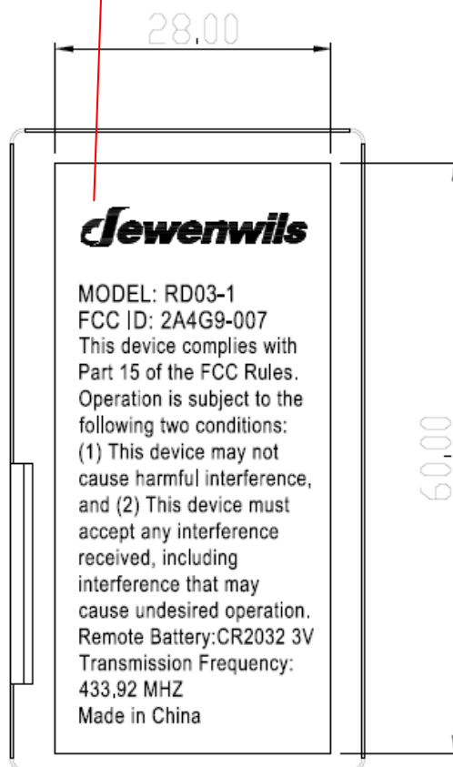
Label Location
