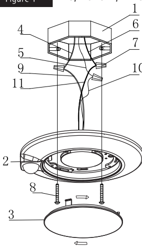
Figure 1 2-3/4 or 3-1/2 inch Inch Junction Box Installation
