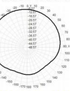
Total(H-XY), Max=-8.57dBi, C/D=12.97
