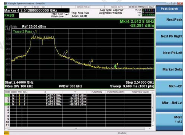
Right bandedge
