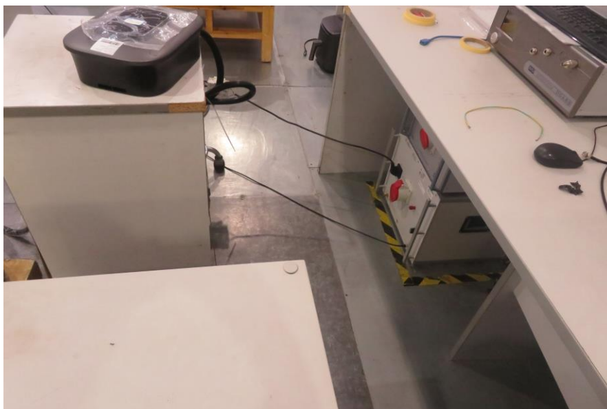
Conducted Disturbance
