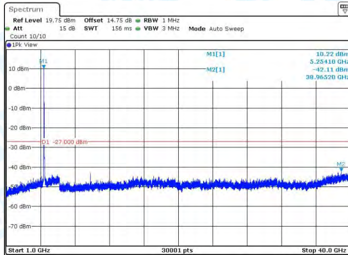
11AC20MIMO_Ant1_5260_1000~40000
