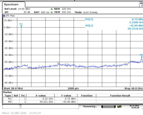
0.03GHz~40GHz
