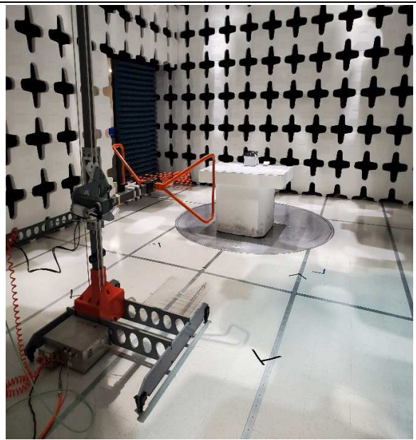
Radiated Emissions Test Below 1GHz Front View
