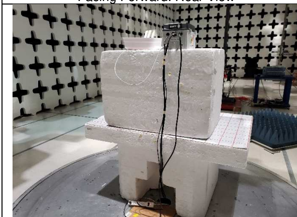
Radiated Emissions Above 1GHz, Antenna Facing Forward. Rear View
