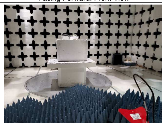
Radiated Emissions Above 1GHz. Antenna Facing Forward. Front View
