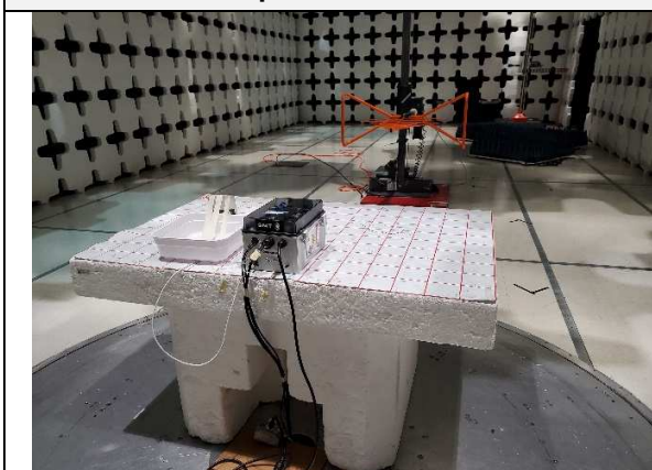
Radiated Emissions Test Below 1GHz. Antenna Facing Forward. Rear View
