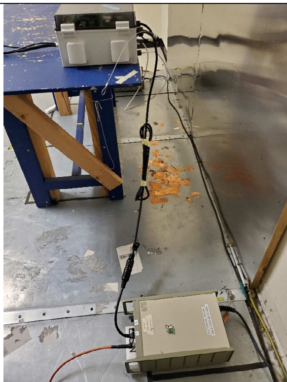
AC Conducted Emissions: Side view
