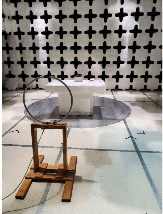
Radiated Emissions Test Below 30MHz Front
