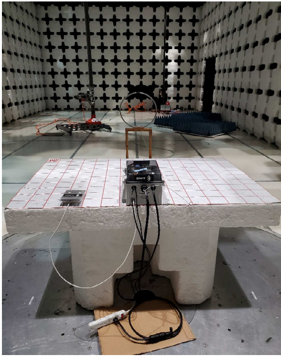
Radiated Emissions Test Below 30MHz Rear
