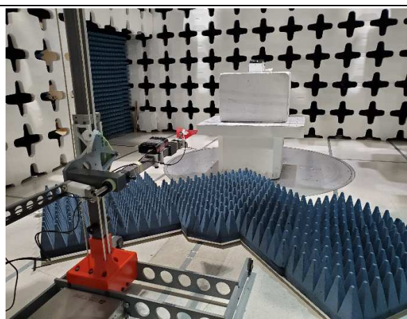
Radiated Emissions Test Above 1GHz. Front View
