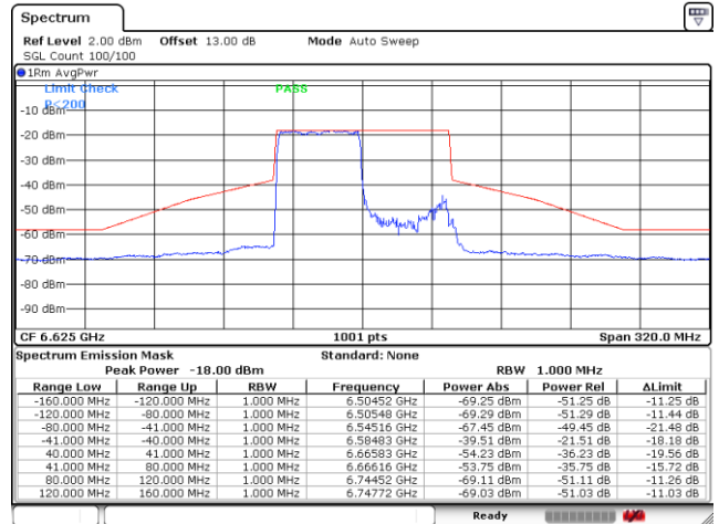
Plot on Channel 6625MHz 484RU65
