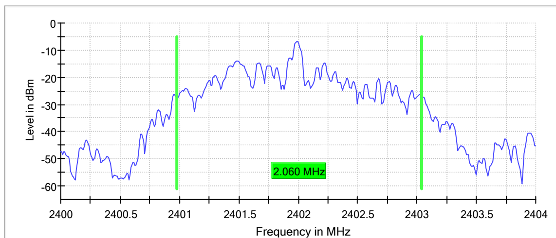
99 % Bandwidth
