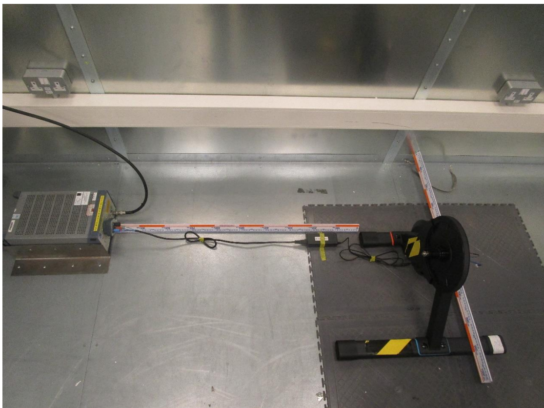
Arrangement for Mains conducted emissions tests
