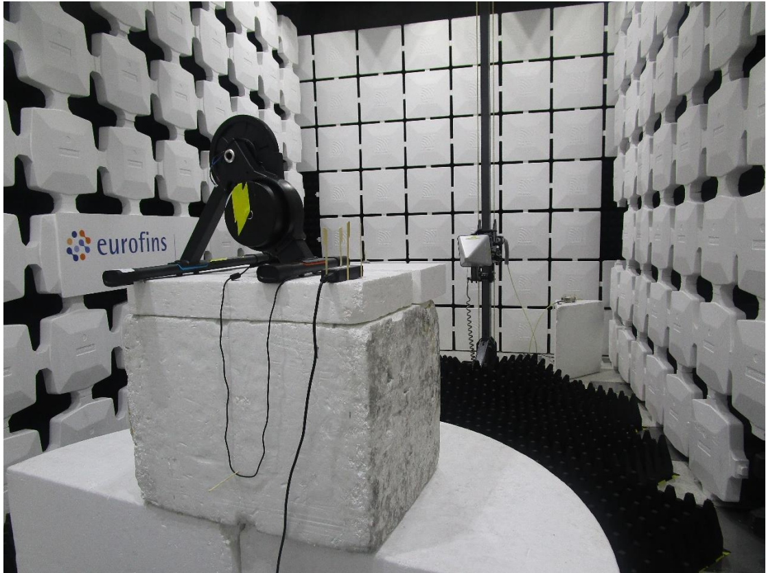
Radiated emissions 1-18GHz 3m distance
