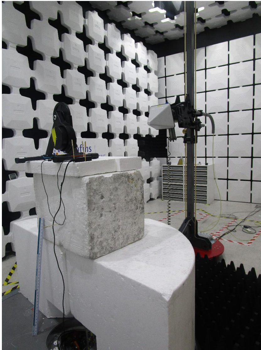
Radiated emissions 1-18GHz 1m distance
