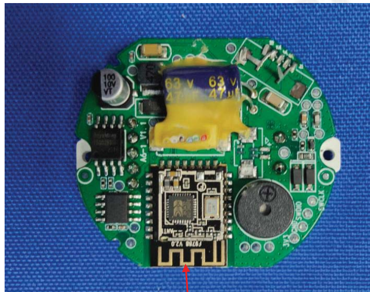
Bluetooth Antenna
