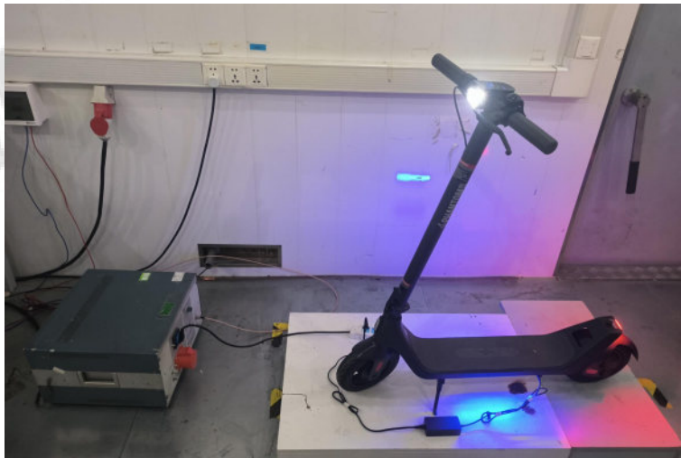
Adapter 2
