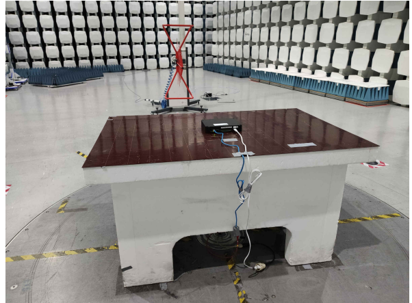
Radiated Emissions 30 – 1000 MHz
