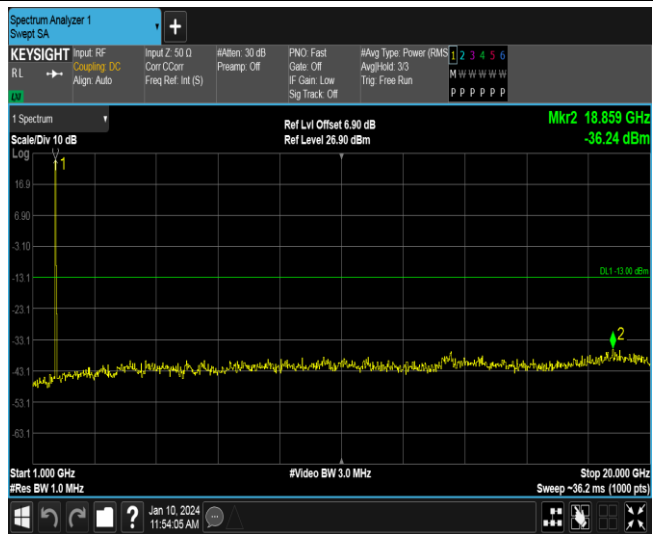
Band66-15MHz-QPSK-132047-1RB#0-Range2:1000~20000MHz
