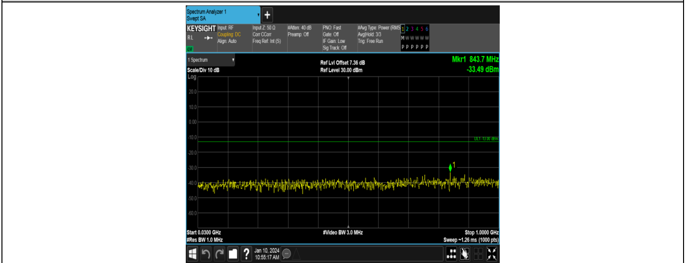
Band66-1.4MHz-QPSK-132665-1RB#0-Range1:30~1000MHz
