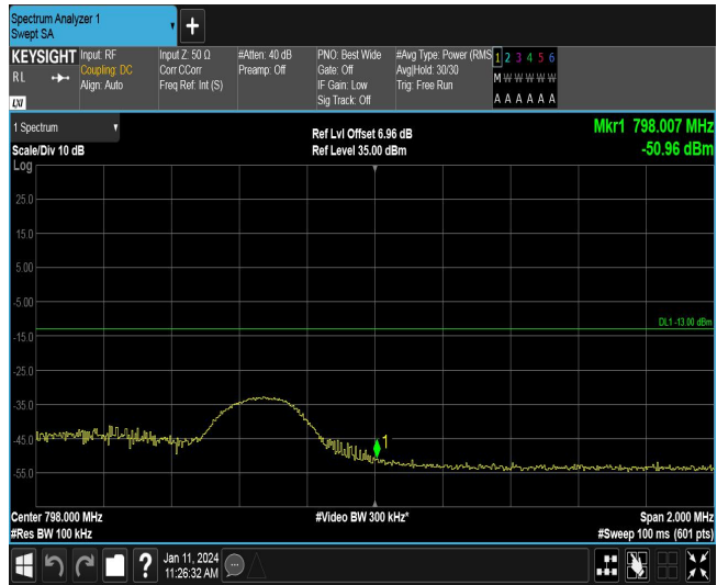
Band14-5MHz-16QAM-23355-1RB#24
