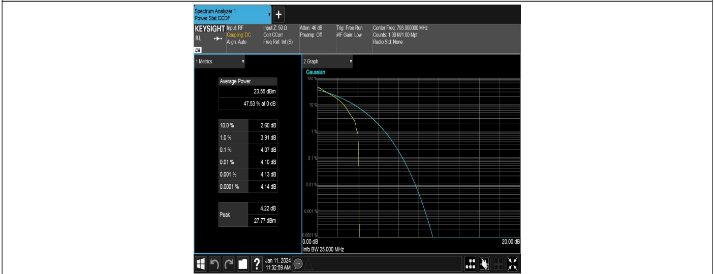
Band14-5MHz-QPSK-23330-25RB#0
