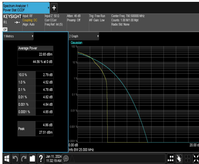
Band14-5MHz-16QAM-23305-25RB#0
