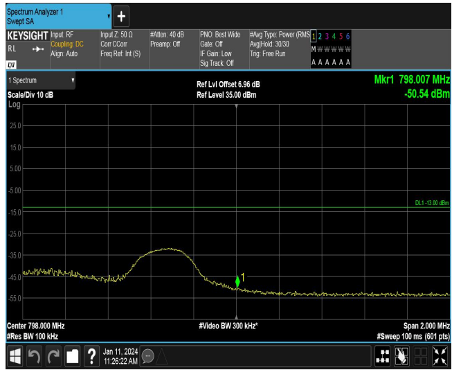
Band14-5MHz-QPSK-23355-1RB#24
