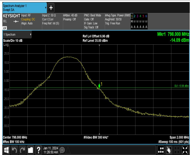
Band14-5MHz-16QAM-23355-1RB#24
