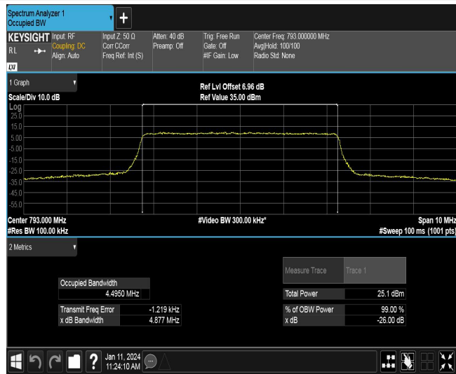
Band 14-5MHz-QPSK-23355-25RB#0
