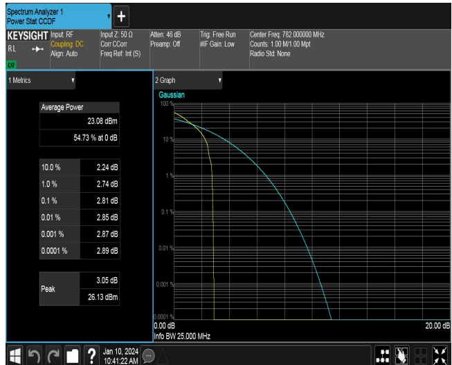
Band13-10MHz-QPSK-23230-50RB#0
