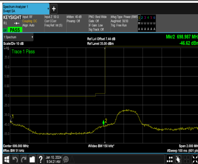
Band12-3MHz-QPSK-23025-1RB#14
