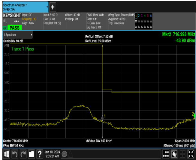
Band12-3MHz-16QAM-23165-1RB#14
