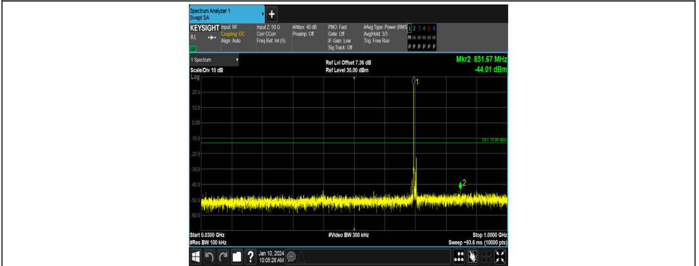
Band12-10MHz-QPSK-23095-1RB#0-Range1:30~1000MHz
