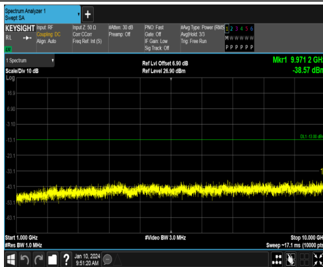
Band12-5MHz-16QAM-23095-1RB#0-Range2:1000~10000MHz
