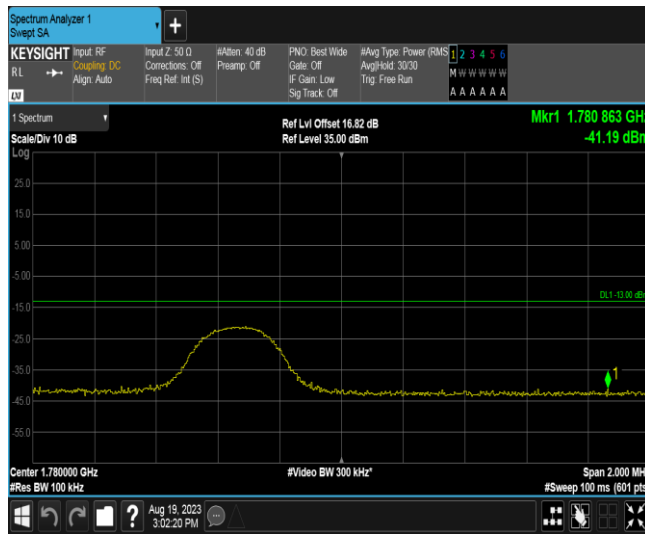
Band66-5MHz-QPSK-132647-1RB#24
