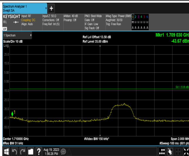
Band66-3MHz-16QAM-131987-1RB#14
