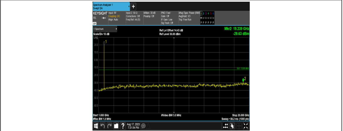
Band4-3MHz-16QAM-19965-1RB#0-Range2:1000~20000MHz
