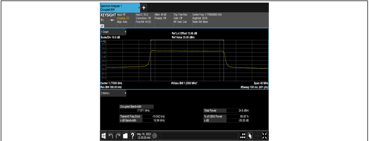
Band66-20MHz-16QAM-132072-100RB#0
