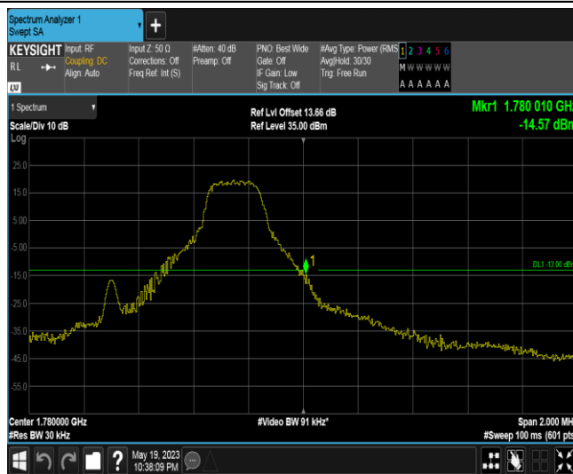
Band66-1.4MHz-QPSK-132665-1RB#5
