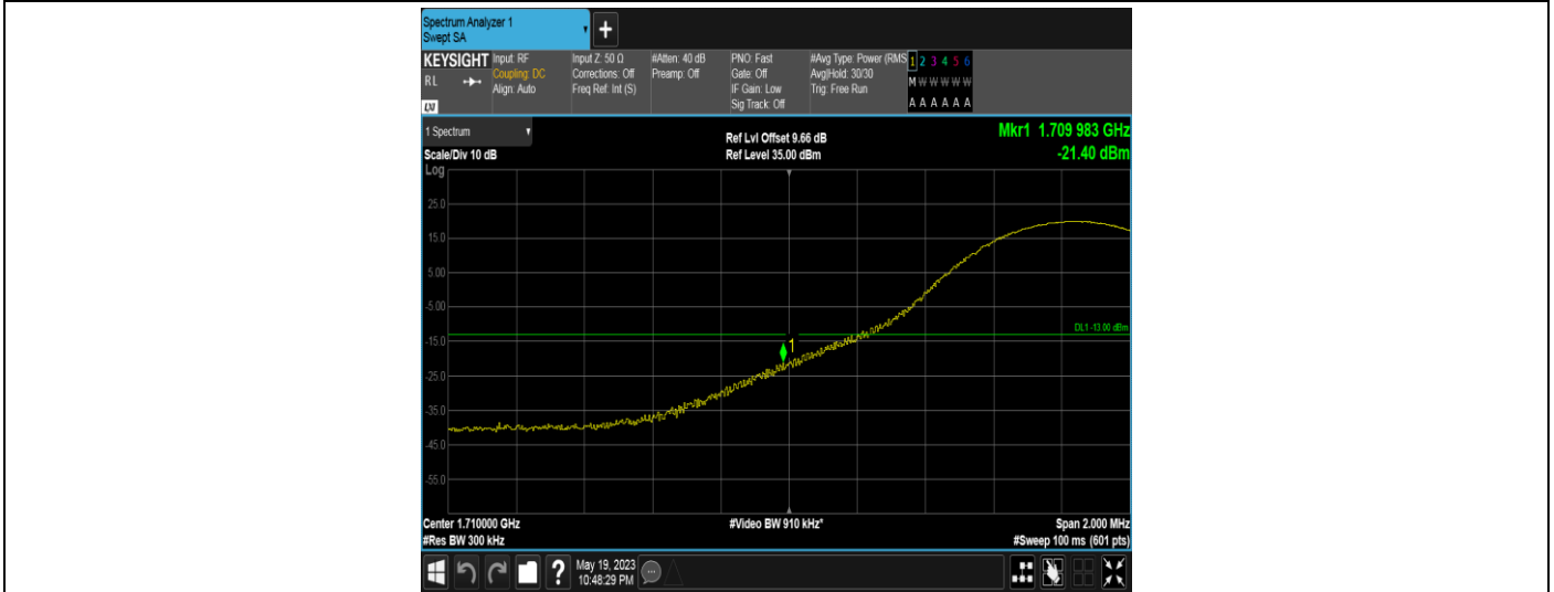
Band66-15MHz-QPSK-132047-1RB#74
