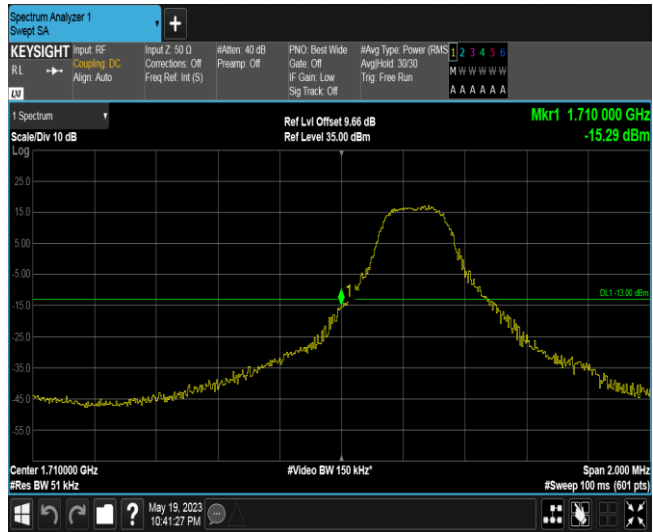
Band66-3MHz-QPSK-131987-1RB#14
