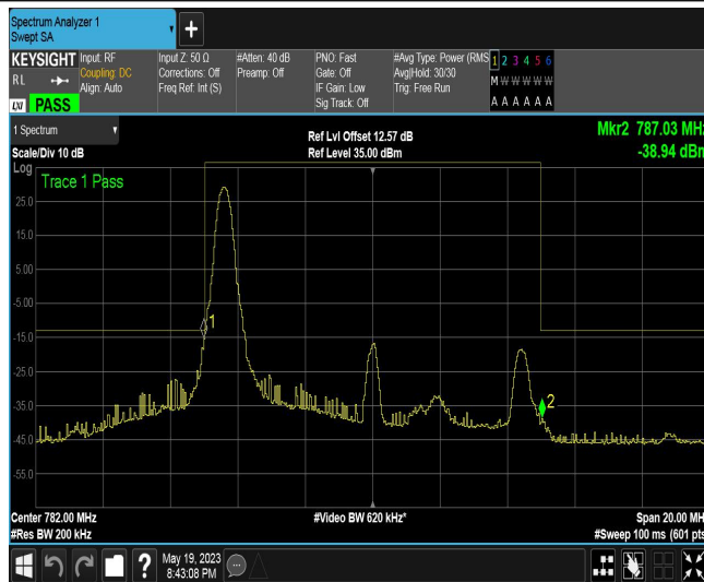
Band13-10MHz-QPSK-23230-1RB#49
