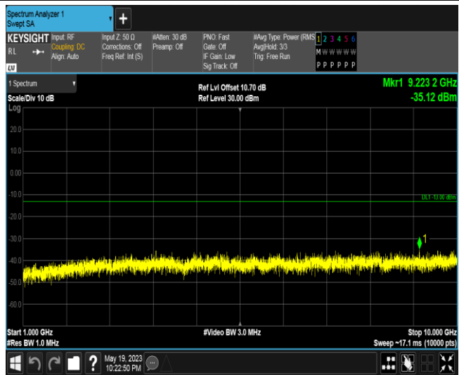
Band13-10MHz-16QAM-23230-1RB#0-Range2:1000~10000MHz
