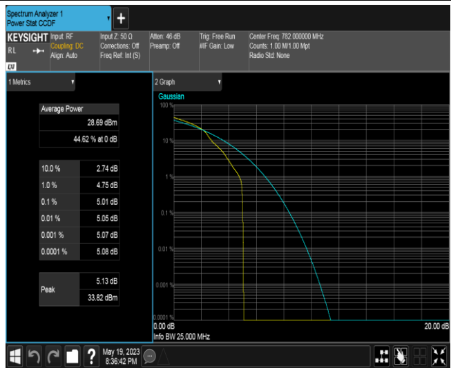
Band13-5MHz-16QAM-23230-1RB#0
