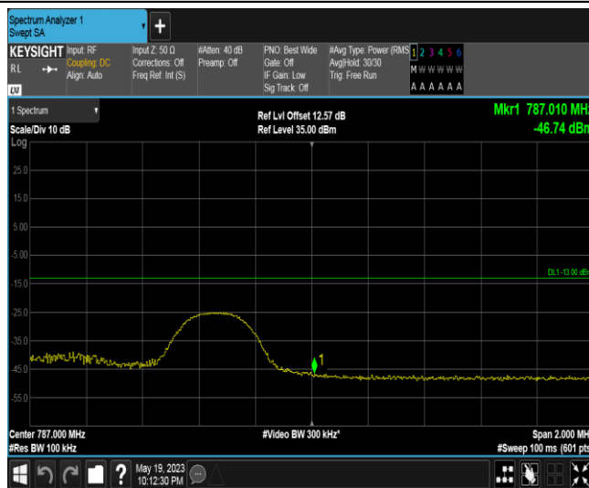
Band13-5MHz-QPSK-23255-1RB#0
