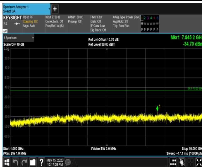
Band5-5MHz-16QAM-20525-1RB#0-Range2:1000~10000MHz
