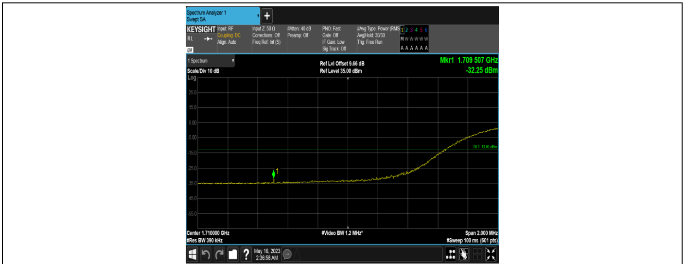
Band4-20MHz-QPSK-20300-1RB#0
