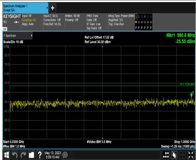
Band2-1.4MHz-QPSK-19193-1RB#0-Range1:30~1000MHz
