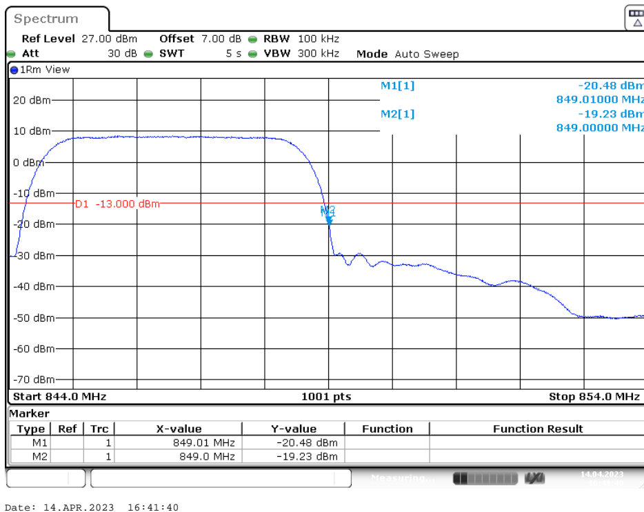
Right Band Edge for RMC (BPSK) Mode
