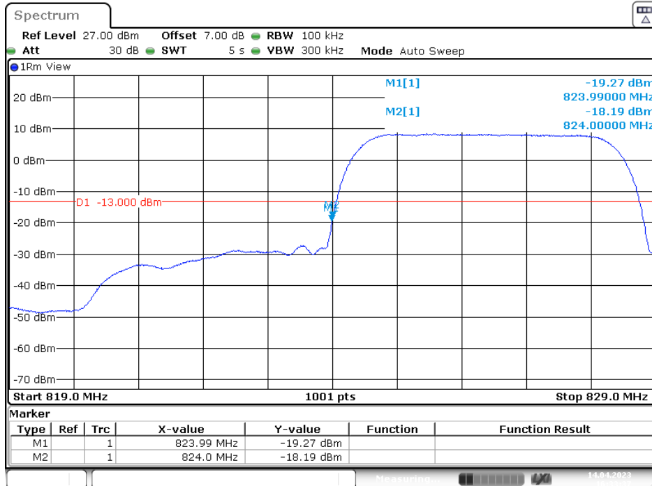
Left Band Edge for RMC (BPSK) Mode
