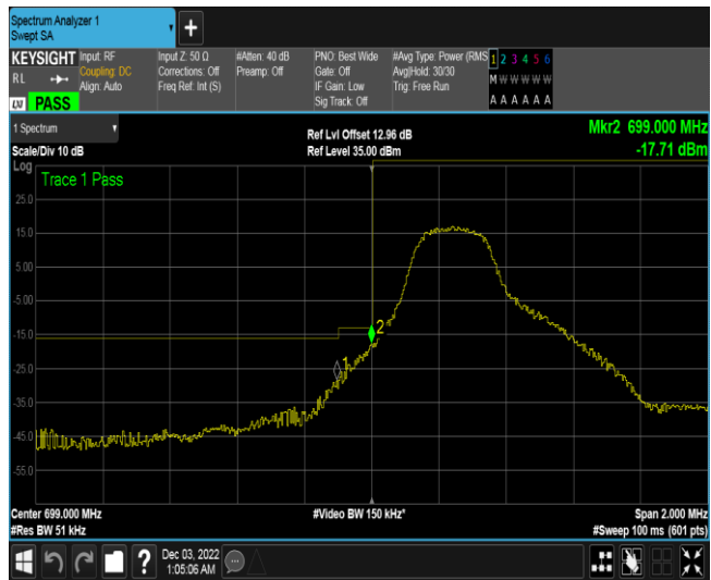
Band12-3MHz-QPSK-23025-1RB#14
