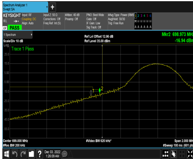
Band12-10MHz-16QAM-23060-1RB#49
