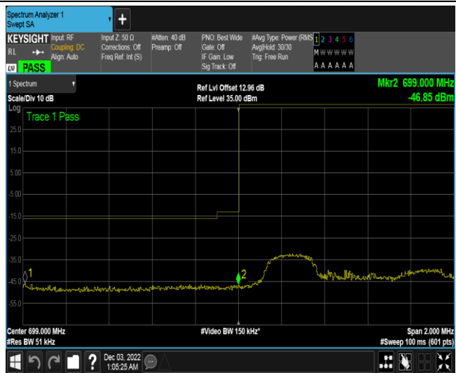
Band12-3MHz-QPSK-23025-1RB#14
