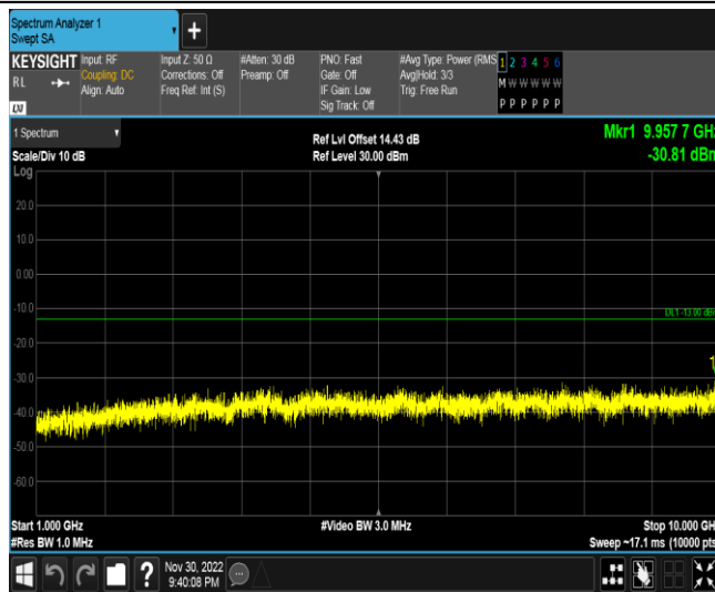
Band12-3MHz-16QAM-23165-1RB#0-Range2:1000~10000MHz
