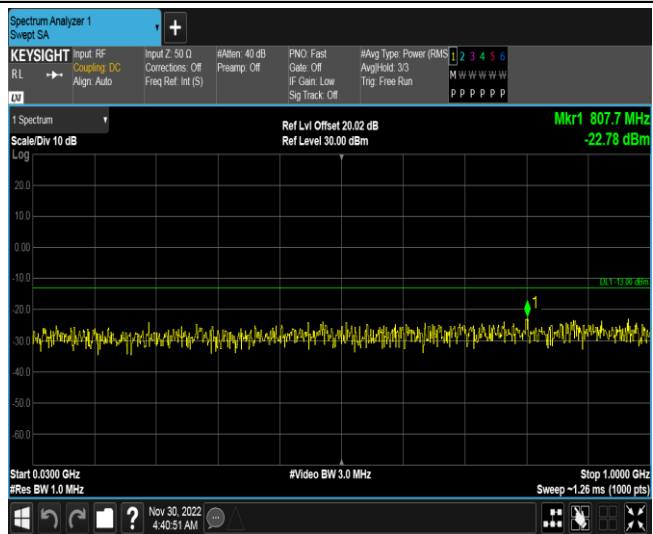
Band4-3MHz-QPSK-20175-1RB#0-Range1:30~1000MHz
