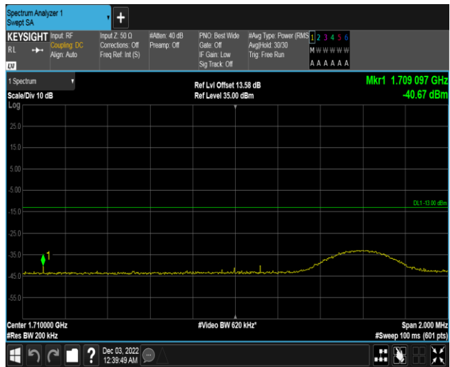
Band4-10MHz-16QAM-20000-50RB#0
