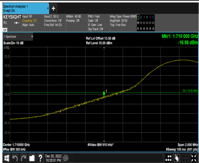
Band4-15MHz-16QAM-20025-1RB#0
