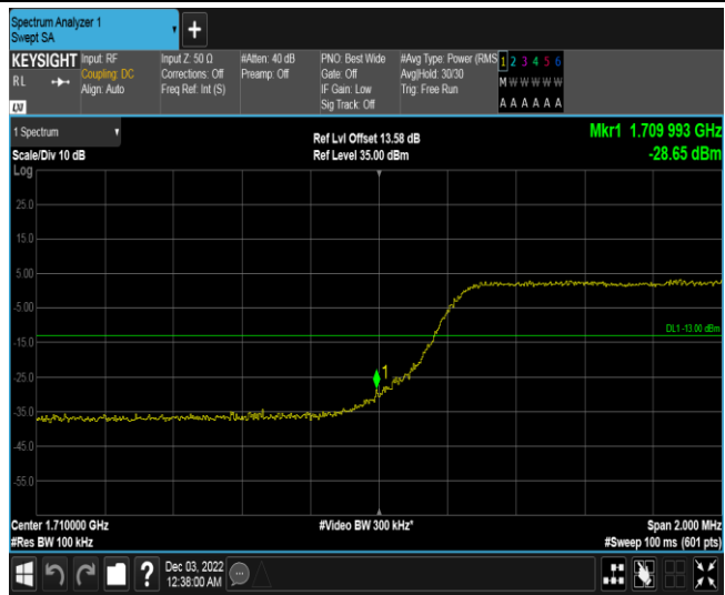
Band4-5MHz-16QAM-20375-1RB#0
