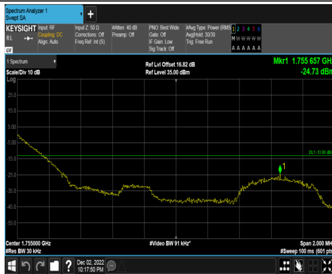
Band4-1.4MHz-16QAM-20393-1RB#0
