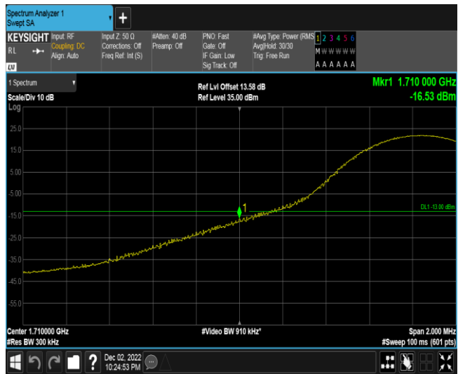
Band4-15MHz-QPSK-20025-1RB#74
