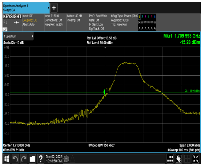
Band4-3MHz-16QAM-19965-1RB#14
