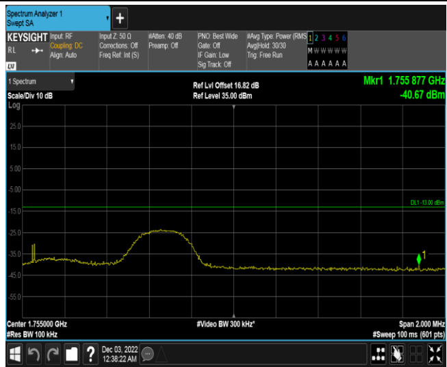
Band4-5MHz-QPSK-20375-1RB#24
