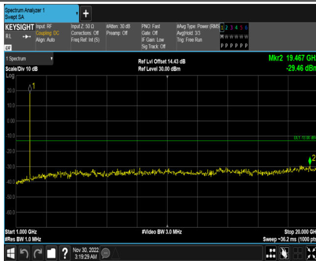
Band2-1.4MHz-16QAM-18900-1RB#0-Range2:1000~20000MHz
