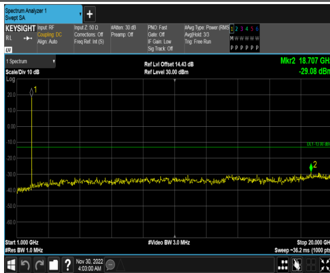
Band2-15MHz-16QAM-19125-1RB#0-Range2:1000~20000MHz
