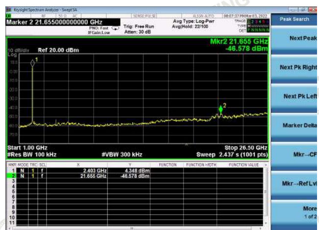
1GHz-26.5GHz
