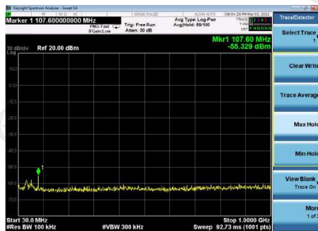
30MHz-1GHz
