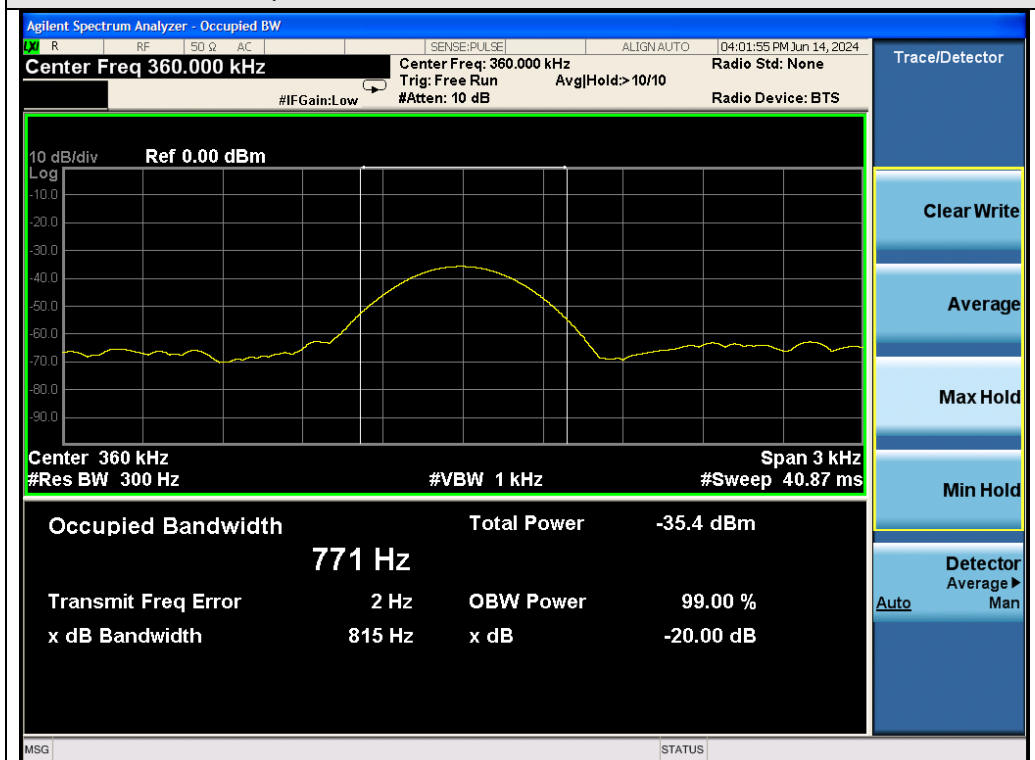
Test_Graph_ASK_Coil ANT_ 360.0kHz _ -20dB Bandwidth
