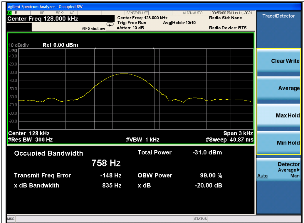
Test_Graph_ASK_Coil ANT_ 128.0kHz _ -20dB Bandwidth
