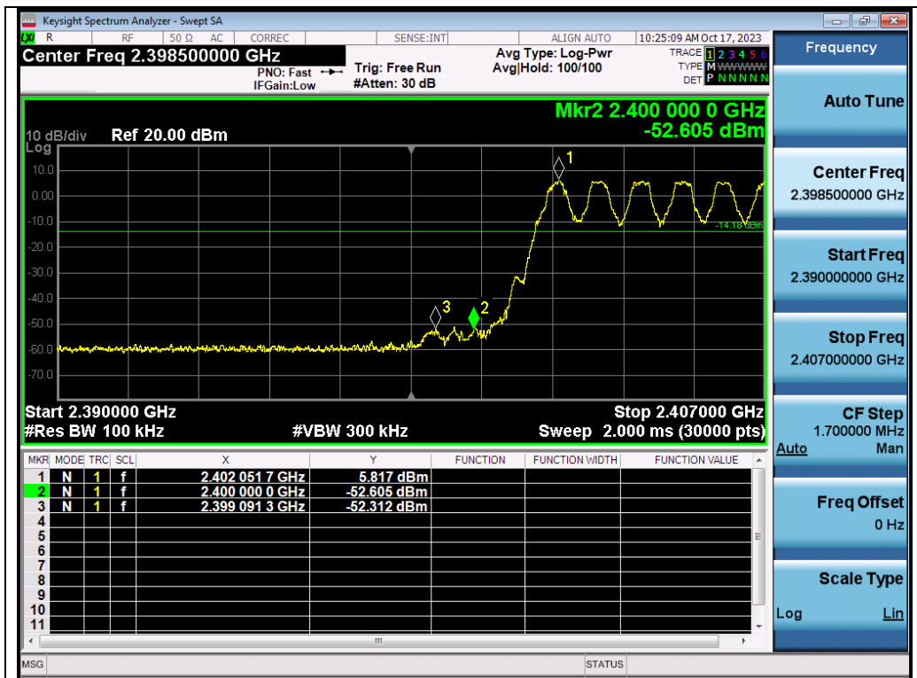
Test_Graph_EDR_HOP_ANT1_NA_1Mbps_Lower Band Edge Emissions
