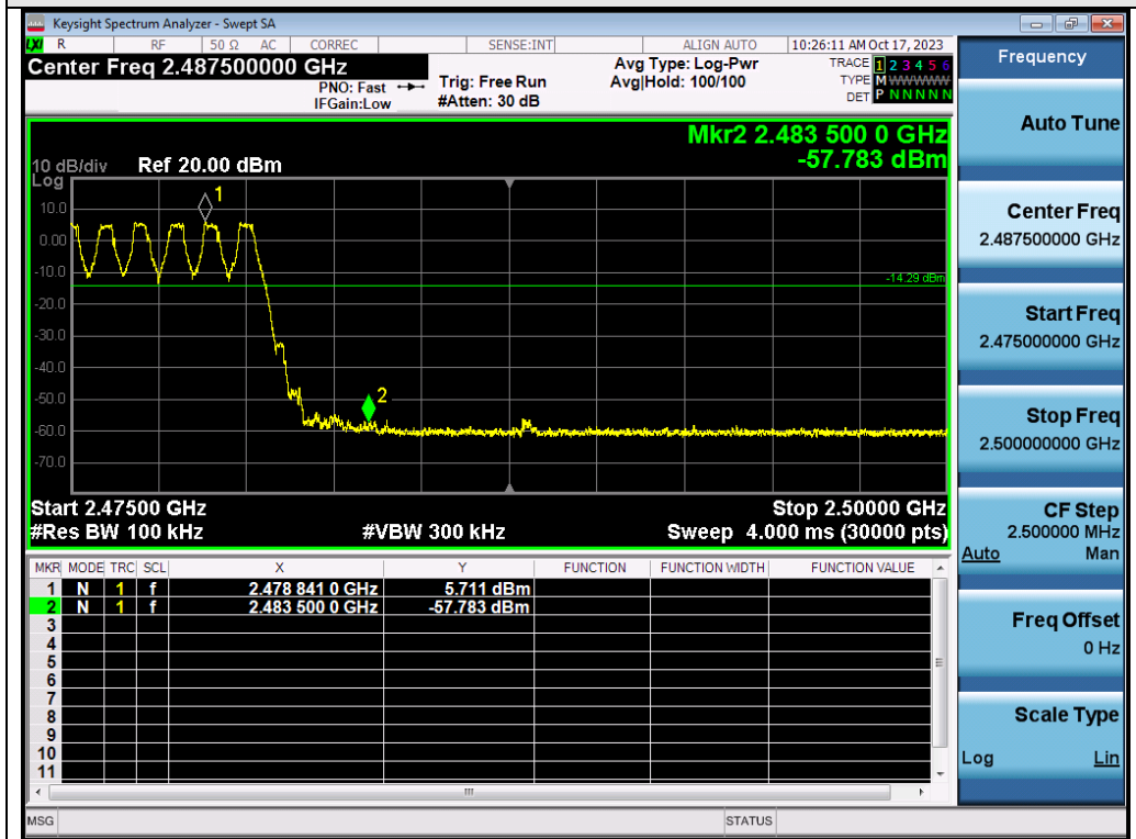
Test_Graph_EDR_HOP_ANT1_NA_1Mbps_Higher Band Edge Emissions
