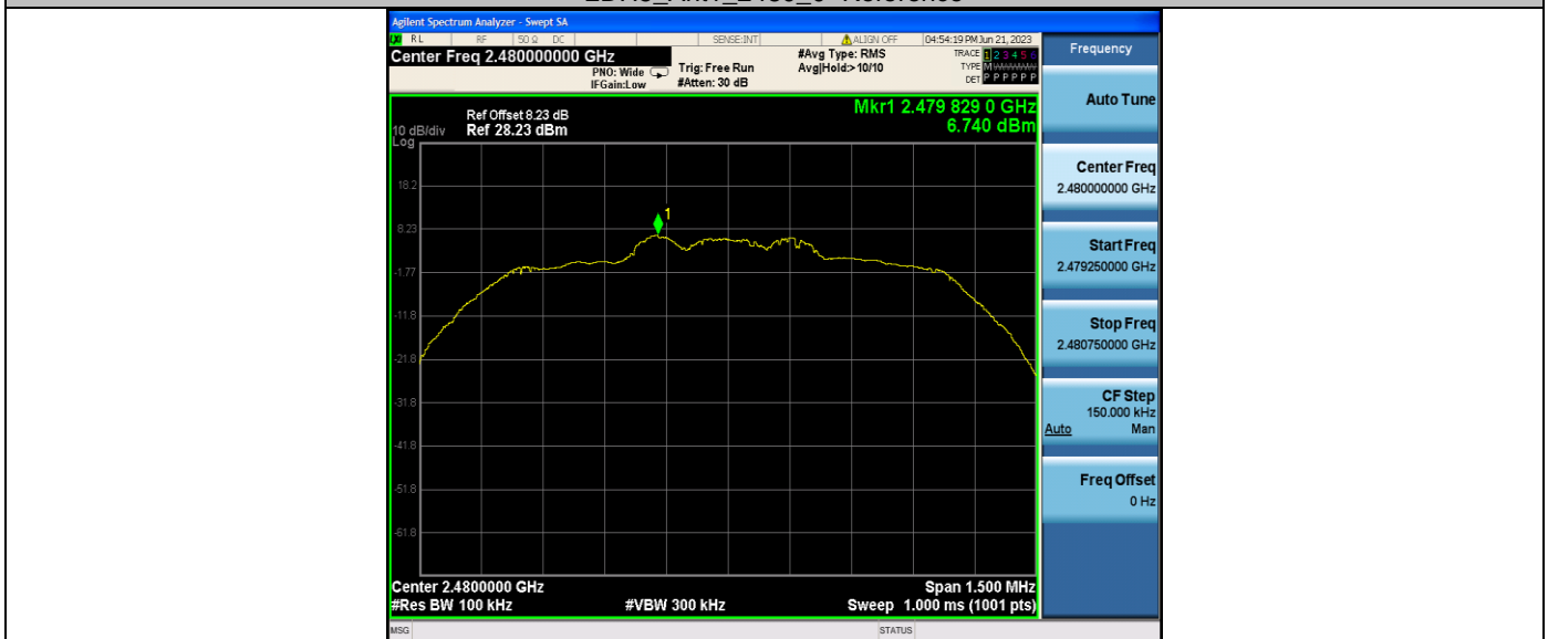
2DH5_Ant1_2480_30~100
