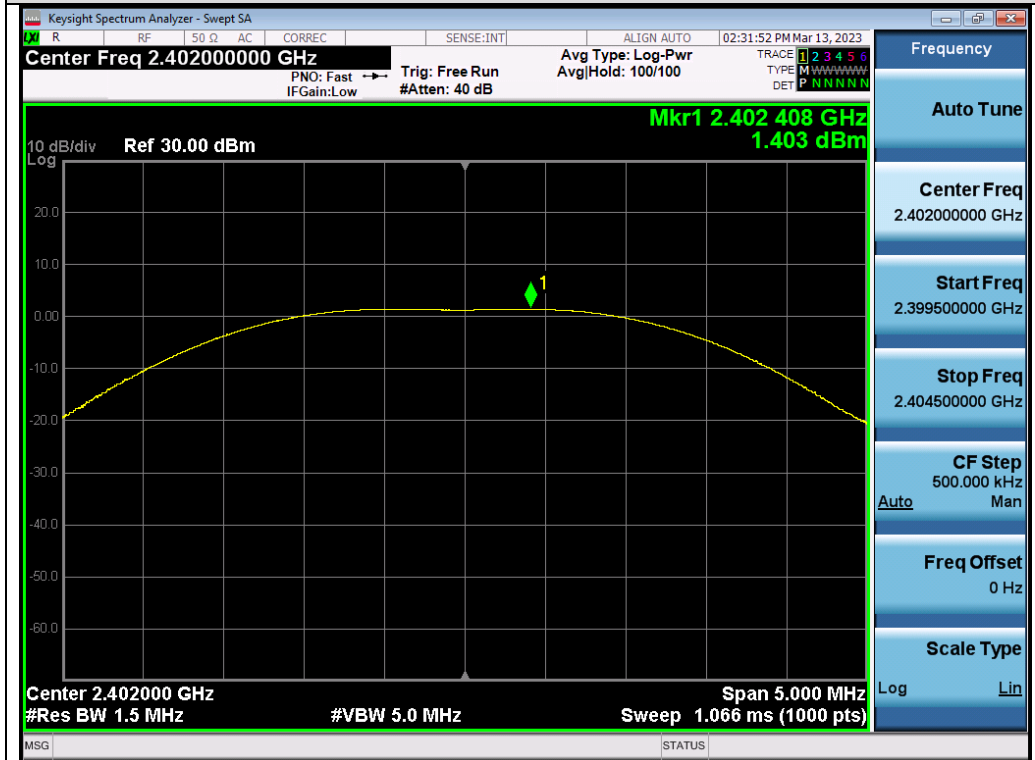
Test_Graph_LE1M_ANT1_2402_2Mbps_Peak Power
