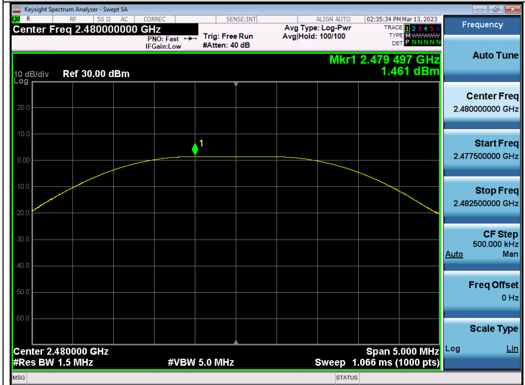
Test_Graph_LE1M_ANT1_2480_2Mbps_Peak Power
