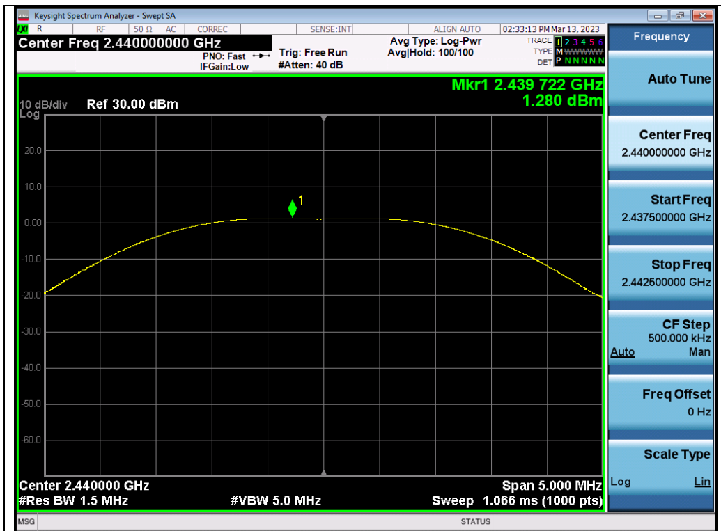
Test_Graph_LE1M_ANT1_2440_2Mbps_Peak Power
