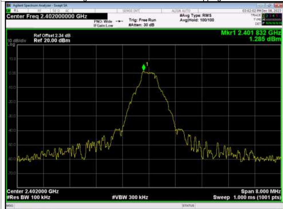
Band Edge NVNT 1-DH1 2402MHz No-Hopping Emission
