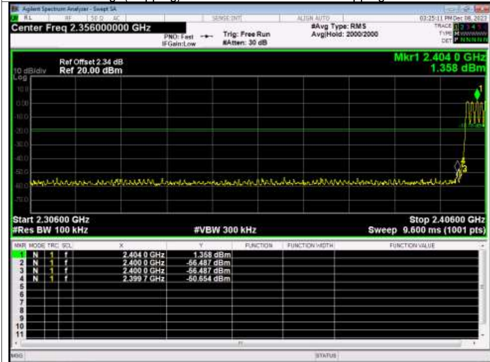
Band Edge(Hopping) NVNT 1-DH1 2402MHz Hopping Emission
