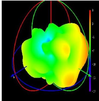
Phi=90 Freq=2440MHz
