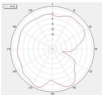
Phi=90 Freq=2440MHz
