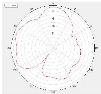
Theta=90 Freq=2440MHz
