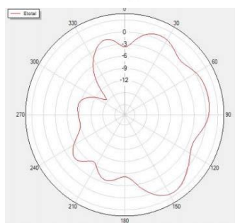
Phi=0 Freq=2440MHz
