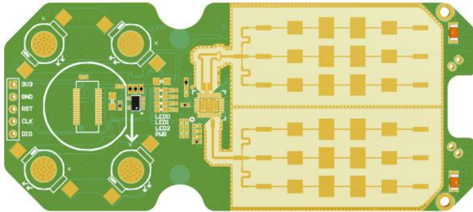
Fig.1 Antenna position
