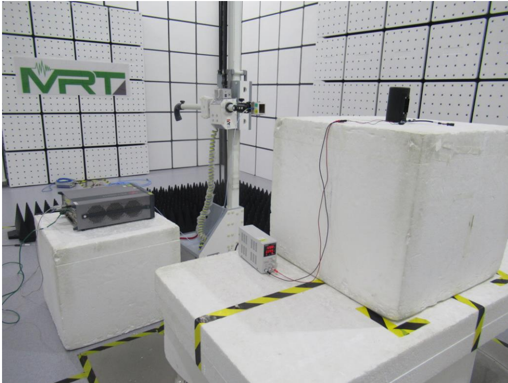
Description: Radiated Band Edge Test Setup
