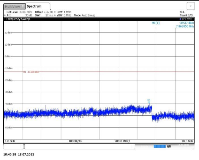
Band5-1.4MHz-16QAM-20643-1RB#0-Range2:1000~10000MHz
