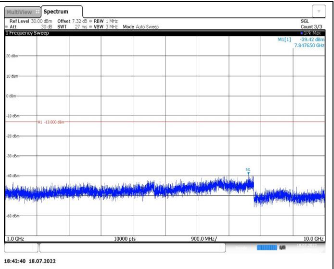
Band5-3MHz-16QAM-20525-1RB#0-Range2:1000~10000MHz
