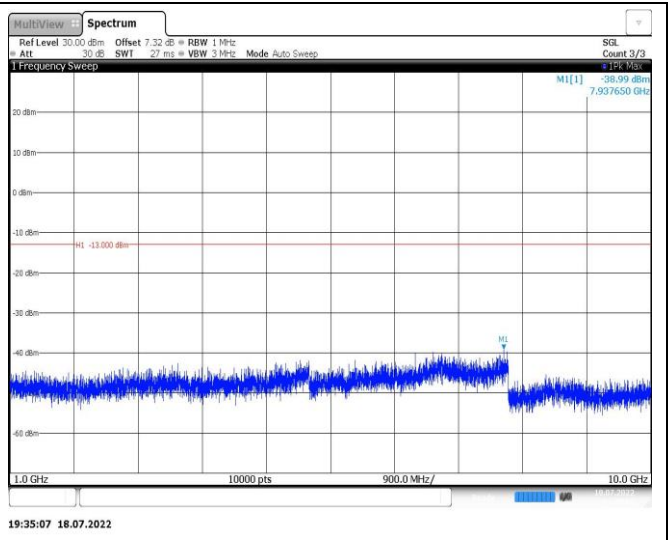
Band12-1.4MHz-16QAM-23095-1RB#0-Range2:1000~10000MHz
