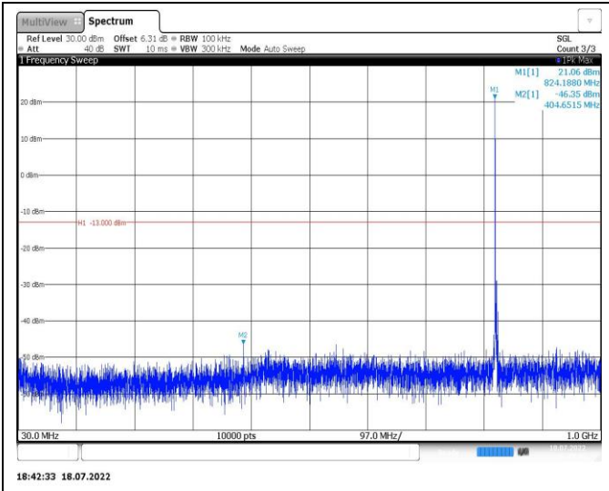
Band5-3MHz-16QAM-20525-1RB#0-Range1:30~1000MHz
