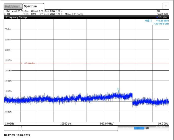
Band5-5MHz-16QAM-20425-1RB#0-Range2:1000~10000MHz
