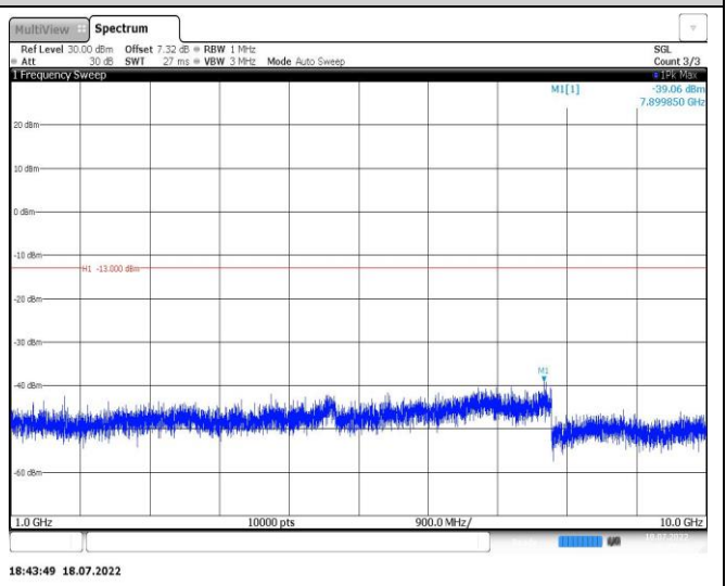
Band5-5MHz-QPSK-20425-1RB#0-Range2:1000~10000MHz
