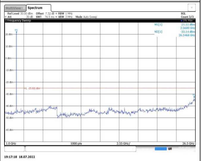
Band7-15MHz-16QAM-20825-1RB#0-Range2:1000~26500MHz
