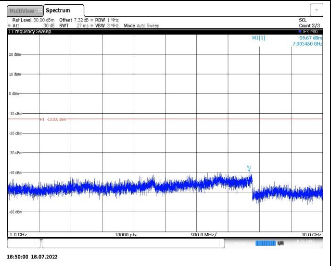
Band5-10MHz-16QAM-20600-1RB#0-Range2:1000~10000MHz
