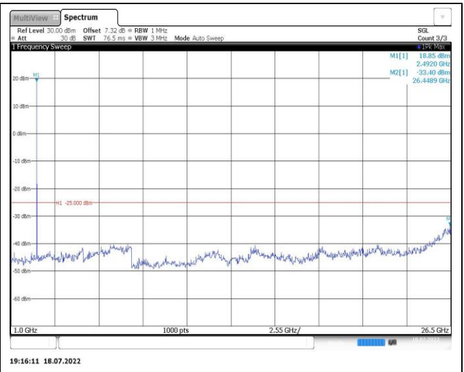
Band7-15MHz-QPSK-21100-1RB#0-Range2:1000~26500MHz
