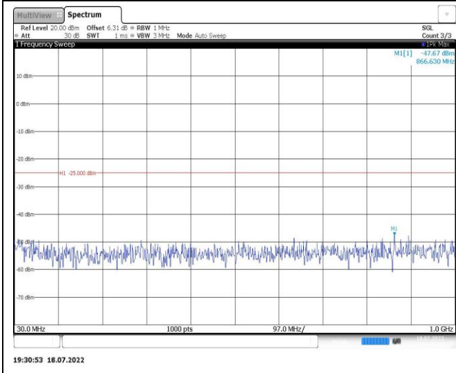
Band7-20MHz-16QAM-21350-1RB#0-Range1:30~1000MHz
