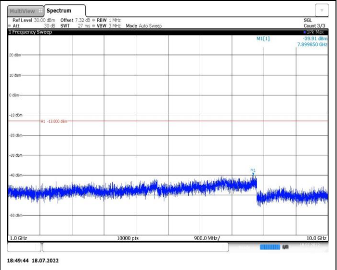
Band5-10MHz-QPSK-20600-1RB#0-Range2:1000~10000MHz
