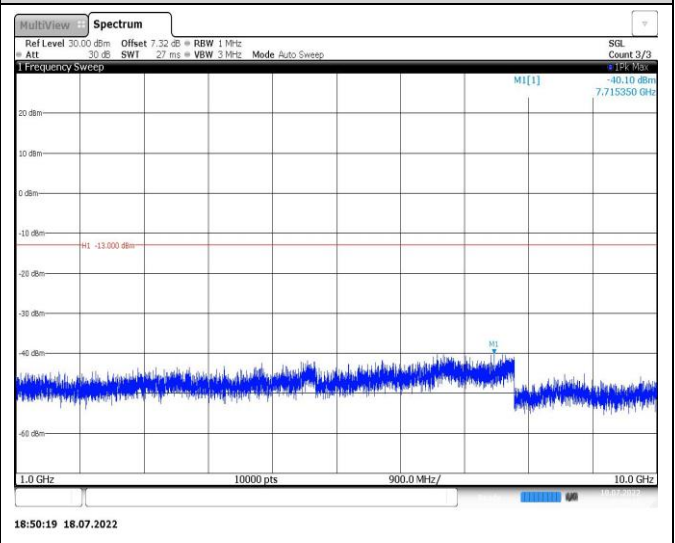
Band5-10MHz-16QAM-20450-1RB#0-Range2:1000~10000MHz
