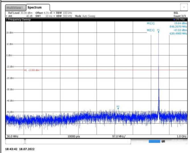
Band5-5MHz-QPSK-20425-1RB#0-Range1:30~1000MHz
