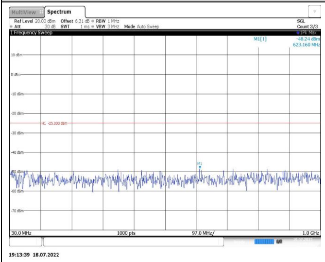
Band7-10MHz-16QAM-21400-1RB#0-Range1:30~1000MHz
