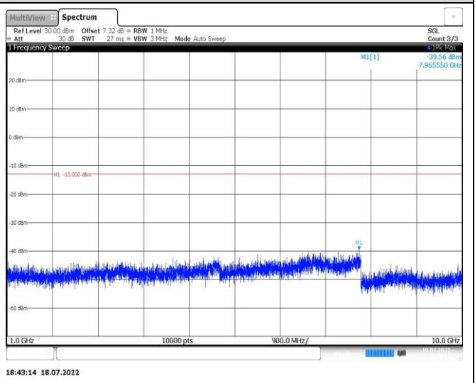
Band5-3MHz-16QAM-20635-1RB#0-Range2:1000~10000MHz
