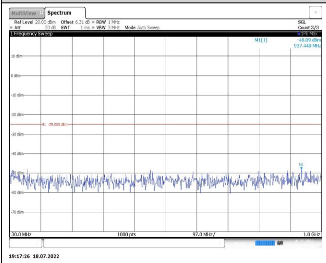
Band7-20MHz-QPSK-20850-1RB#0-Range1:30~1000MHz
