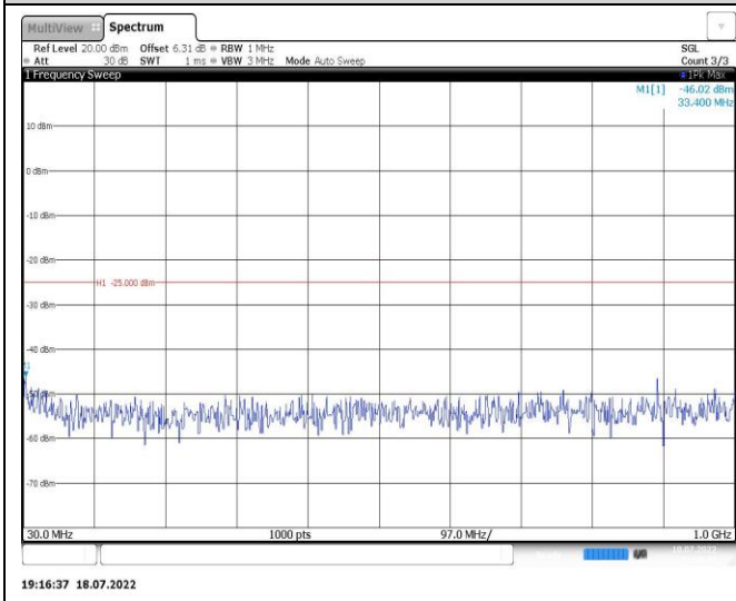
Band7-15MHz-QPSK-21375-1RB#0-Range1:30~1000MHz
