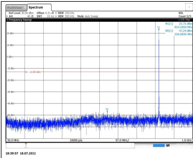
Band5-1.4MHz-16QAM-20525-1RB#0-Range1:30~1000MHz
