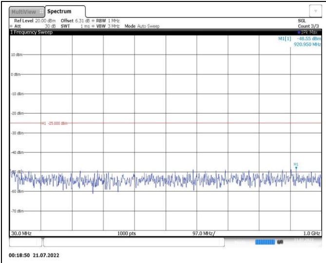
Band7-5MHz-16QAM-21100-1RB#0-Range1:30~1000MHz
