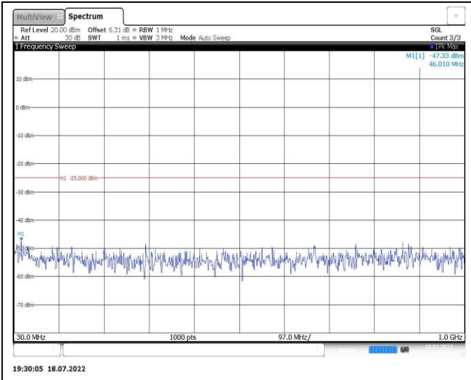
Band7-20MHz-QPSK-21100-1RB#0-Range1:30~1000MHz
