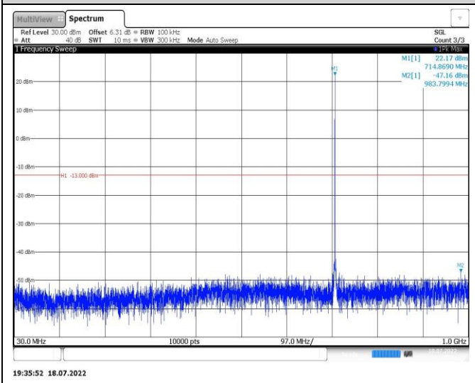
Band12-1.4MHz-16QAM-23017-1RB#0-Range1:30~1000MHz
