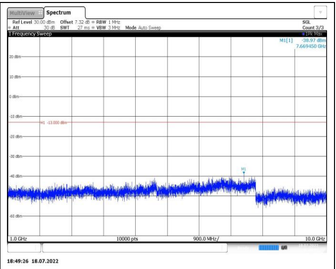
Band5-10MHz-16QAM-20525-1RB#0-Range2:1000~10000MHz
