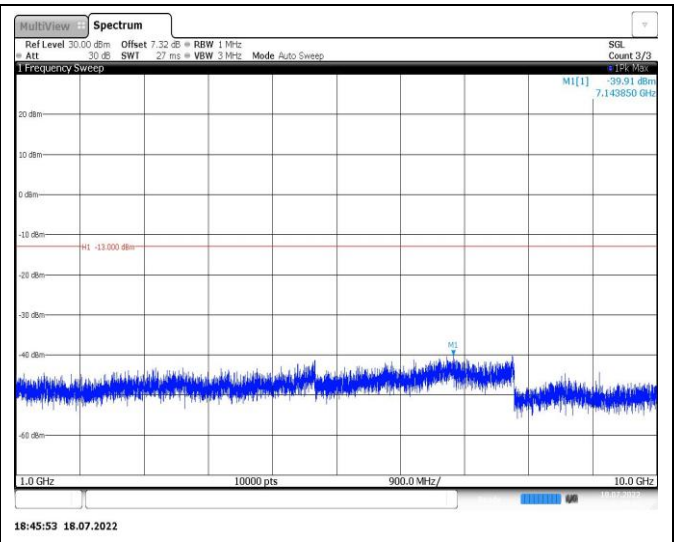
Band5-5MHz-QPSK-20525-1RB#0-Range2:1000~10000MHz
