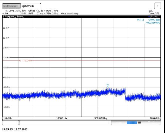
Band12-1.4MHz-QPSK-23173-1RB#0-Range2:1000~10000MHz
