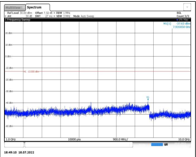
Band5-10MHz-QPSK-20525-1RB#0-Range2:1000~10000MHz
