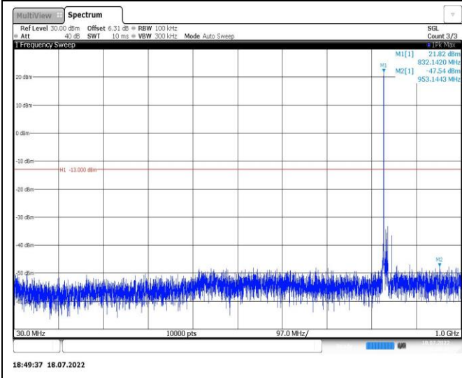
Band5-10MHz-QPSK-20600-1RB#0-Range1:30~1000MHz
