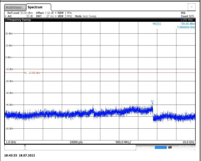
Band5-3MHz-16QAM-20415-1RB#0-Range2:1000~10000MHz
