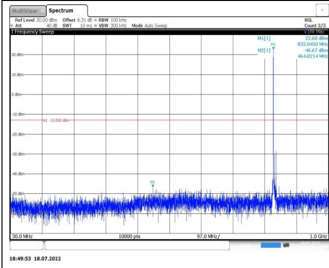
Band5-10MHz-16QAM-20600-1RB#0-Range1:30~1000MHz
