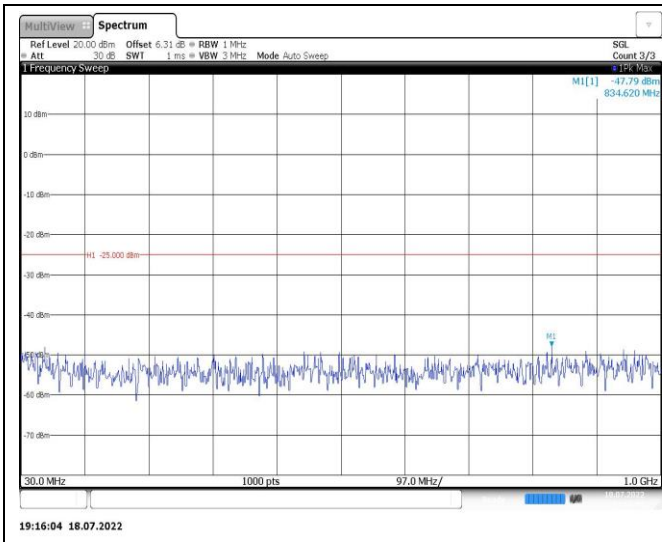
Band7-15MHz-QPSK-21100-1RB#0-Range1:30~1000MHz
