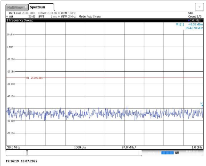
Band7-15MHz-16QAM-21100-1RB#0-Range1:30~1000MHz
