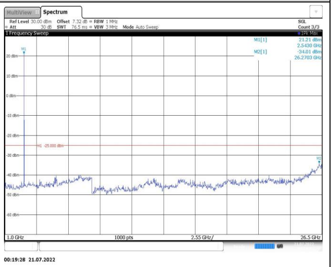
Band7-5MHz-16QAM-21425-1RB#0-Range2:1000~26500MHz
