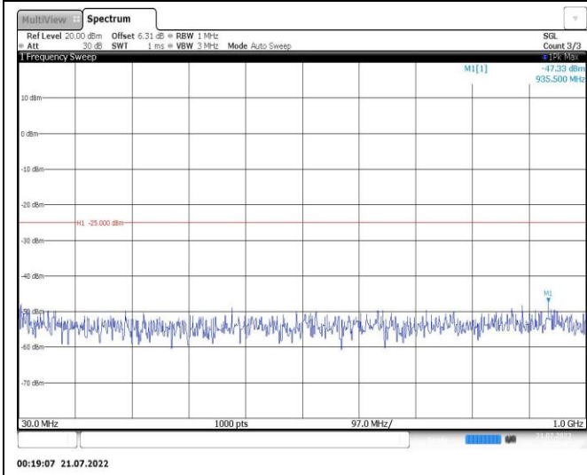
Band7-5MHz-QPSK-21425-1RB#0-Range1:30~1000MHz
