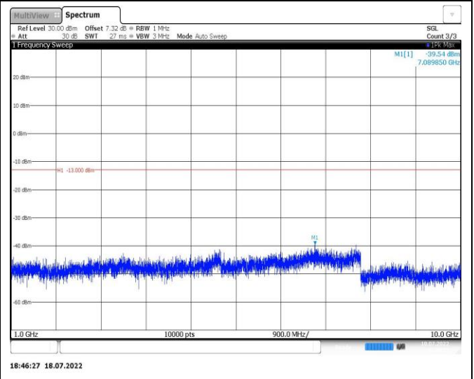
Band5-5MHz-QPSK-20625-1RB#0-Range2:1000~10000MHz
