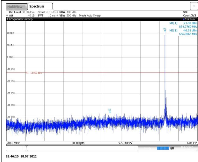
Band5-5MHz-QPSK-20625-1RB#0-Range1:30~1000MHz
