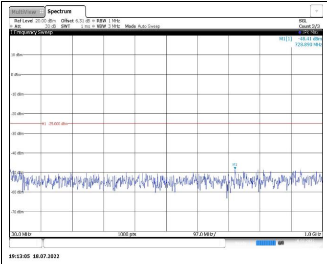
Band7-10MHz-16QAM-21100-1RB#0-Range1:30~1000MHz
