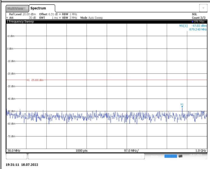
Band7-20MHz-16QAM-20850-1RB#0-Range1:30~1000MHz
