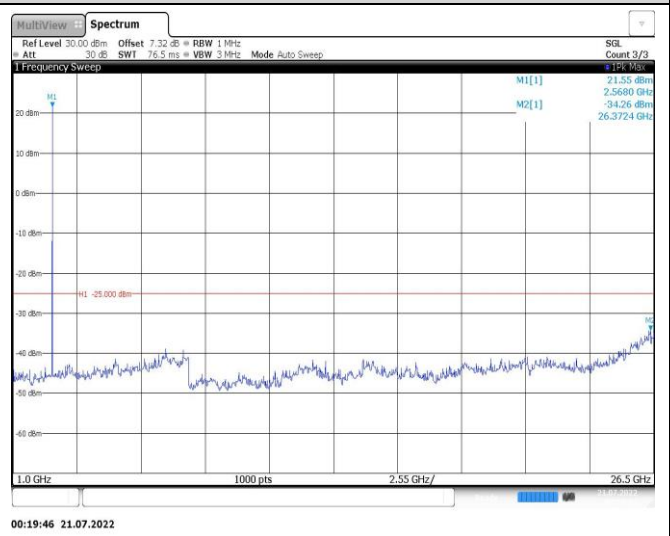
Band7-5MHz-16QAM-20775-1RB#0-Range2:1000~26500MHz
