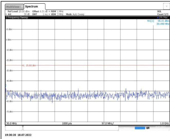
Band7-20MHz-16QAM-21100-1RB#0-Range1:30~1000MHz
