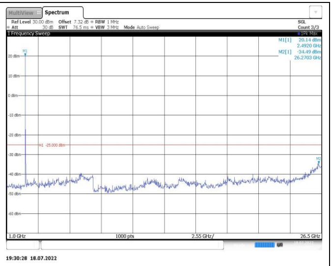
Band7-20MHz-16QAM-21100-1RB#0-Range2:1000~26500MHz
