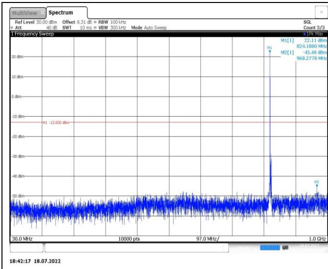
Band5-3MHz-QPSK-20525-1RB#0-Range1:30~1000MHz
