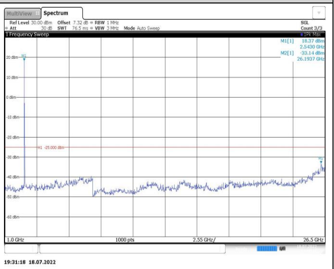
Band7-20MHz-16QAM-20850-1RB#0-Range2:1000~26500MHz
