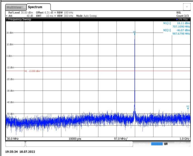
Band12-1.4MHz-16QAM-23173-1RB#0-Range1:30~1000MHz
