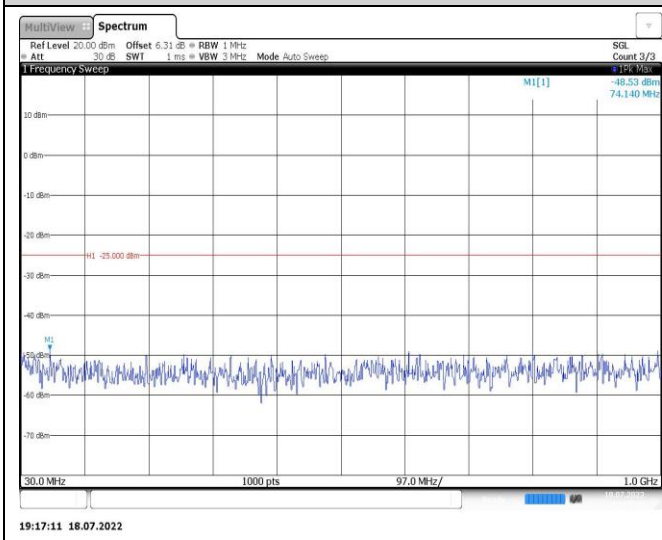
Band7-15MHz-16QAM-20825-1RB#0-Range1:30~1000MHz
