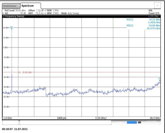
Band7-5MHz-16QAM-21100-1RB#0-Range2:1000~26500MHz
