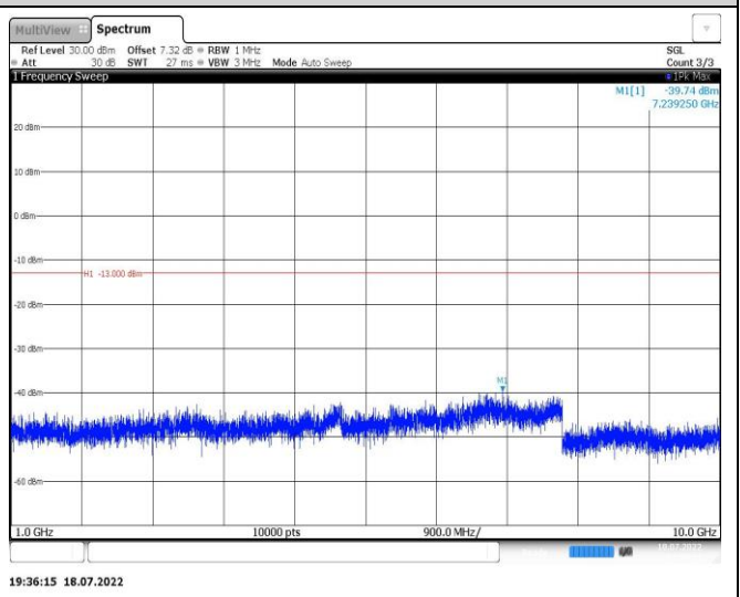
Band12-3MHz-QPSK-23025-1RB#0-Range2:1000~10000MHz
