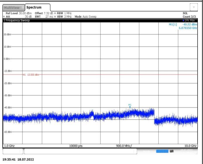
Band12-1.4MHz-16QAM-23173-1RB#0-Range2:1000~10000MHz
