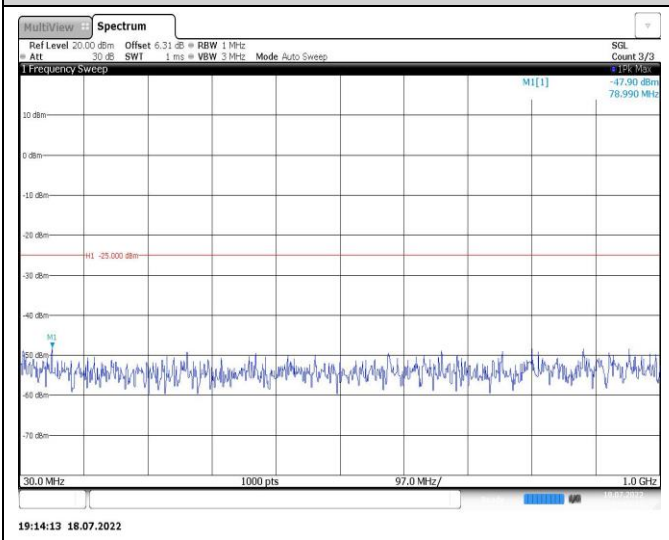
Band7-15MHz-QPSK-20825-1RB#0-Range1:30~1000MHz
