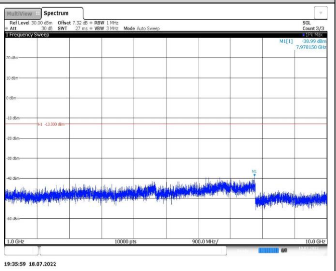
Band12-1.4MHz-16QAM-23017-1RB#0-Range2:1000~10000MHz
