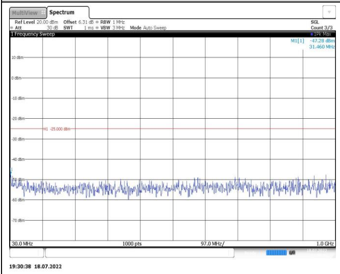
Band7-20MHz-QPSK-21350-1RB#0-Range1:30~1000MHz
