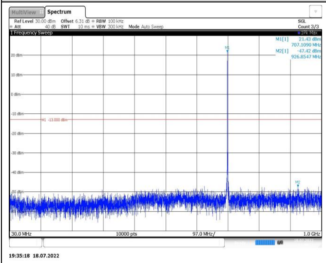
Band12-1.4MHz-QPSK-23173-1RB#0-Range1:30~1000MHz
