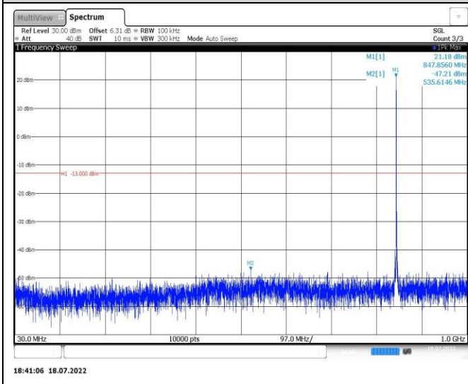
Band5-3MHz-QPSK-20415-1RB#0-Range1:30~1000MHz
