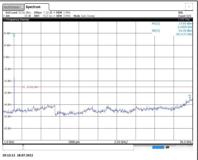
Band7-10MHz-16QAM-21100-1RB#0-Range2:1000~26500MHz
