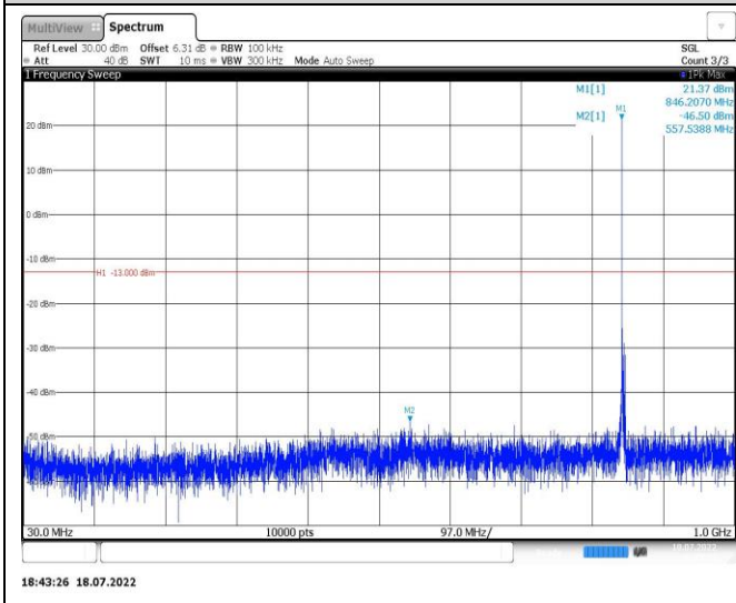
Band5-3MHz-16QAM-20415-1RB#0-Range1:30~1000MHz
