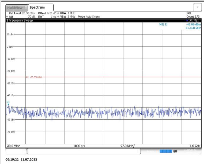
Band7-5MHz-16QAM-21425-1RB#0-Range1:30~1000MHz
