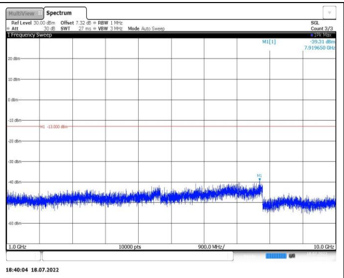
Band5-1.4MHz-16QAM-20525-1RB#0-Range2:1000~10000MHz
