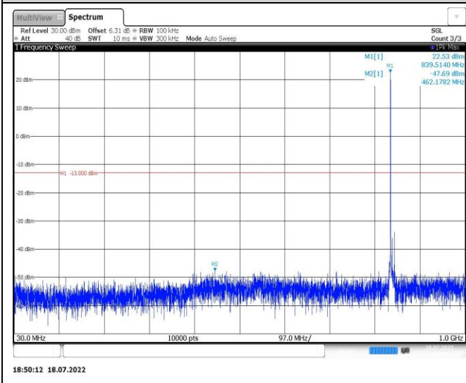
Band5-10MHz-16QAM-20450-1RB#0-Range1:30~1000MHz
