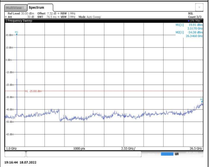
Band7-15MHz-QPSK-21375-1RB#0-Range2:1000~26500MHz
