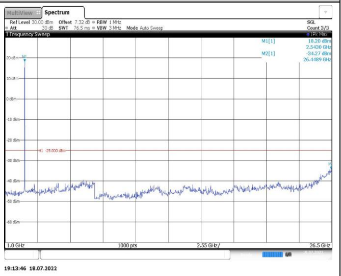
Band7-10MHz-16QAM-21400-1RB#0-Range2:1000~26500MHz
