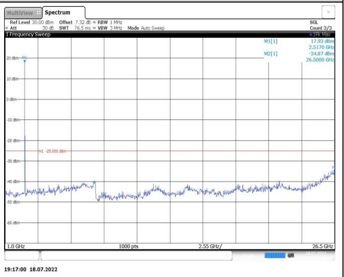
Band7-15MHz-16QAM-21375-1RB#0-Range2:1000~26500MHz
