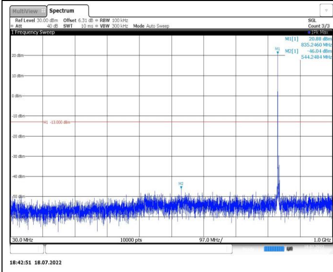
Band5-3MHz-QPSK-20635-1RB#0-Range1:30~1000MHz
