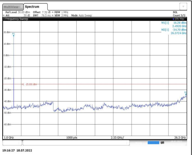
Band7-15MHz-16QAM-21100-1RB#0-Range2:1000~26500MHz
