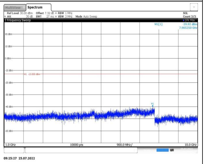
Band26-15MHz-QPSK-26915-1RB#0-Range2:1000~10000MHz
