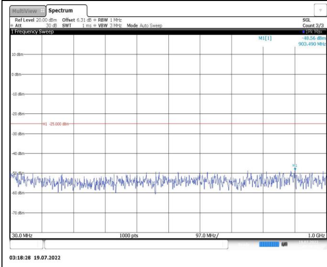
Band38-15MHz-16QAM-37825-1RB#0-Range1:30~1000MHz
