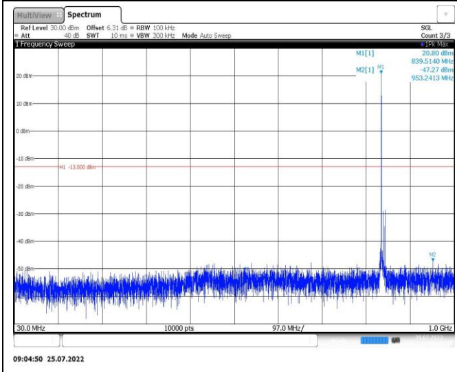
Band26-15MHz-QPSK-26865-1RB#0-Range1:30~1000MHz
