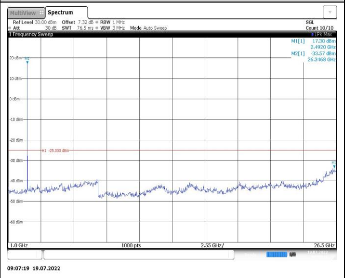
Band41-10MHz-16QAM-40620-1RB#0-Range2:1000~26500MHz
