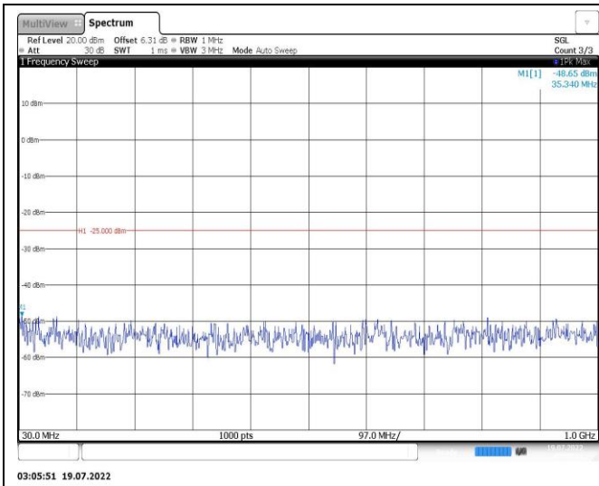
Band38-10MHz-QPSK-38200-1RB#0-Range1:30~1000MHz
