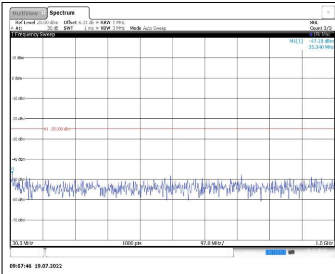
Band41-10MHz-16QAM-41540-1RB#0-Range1:30~1000MHz
