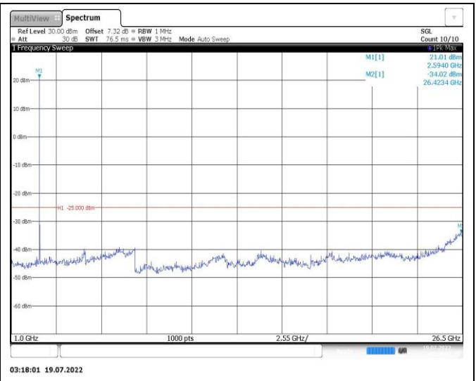
Band38-15MHz-QPSK-38175-1RB#0-Range2:1000~26500MHz
