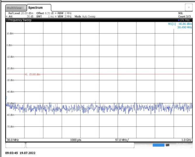
Band41-5MHz-QPSK-40620-1RB#0-Range1:30~1000MHz
