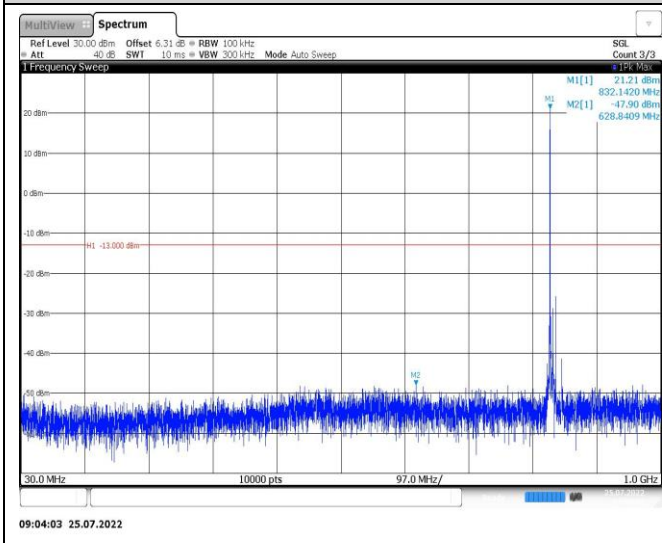
Band26-10MHz-QPSK-26990-1RB#0-Range1:30~1000MHz
