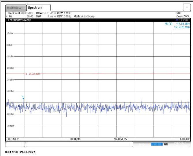
Band38-15MHz-QPSK-38000-1RB#0-Range1:30~1000MHz
