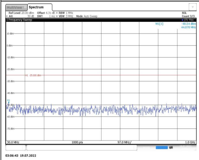
Band38-15MHz-QPSK-37825-1RB#0-Range1:30~1000MHz
