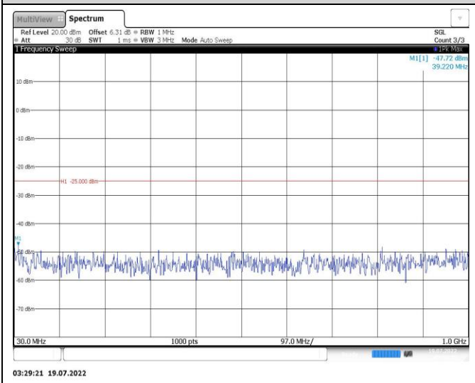
Band38-20MHz-QPSK-38000-1RB#0-Range1:30~1000MHz
