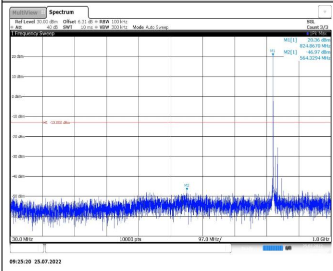
Band26-15MHz-QPSK-26915-1RB#0-Range1:30~1000MHz
