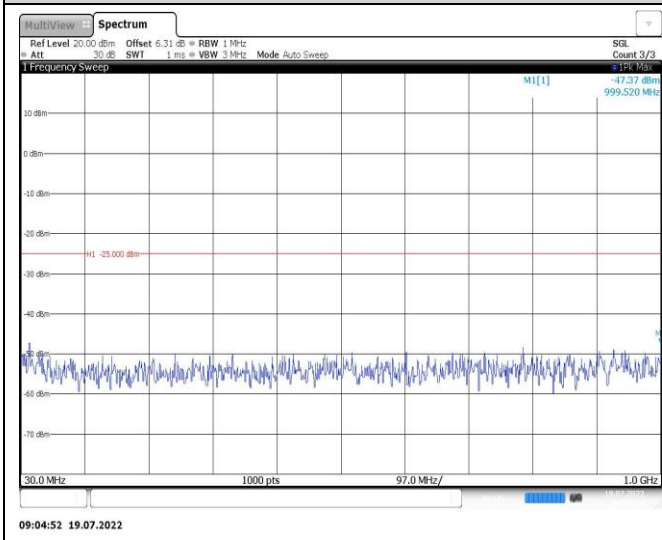
Band41-5MHz-16QAM-39675-1RB#0-Range1:30~1000MHz
