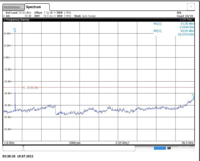
Band38-20MHz-16QAM-38150-1RB#0-Range2:1000~26500MHz
