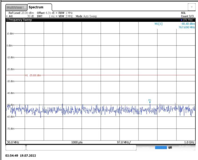
Band38-10MHz-QPSK-37800-1RB#0-Range1:30~1000MHz
