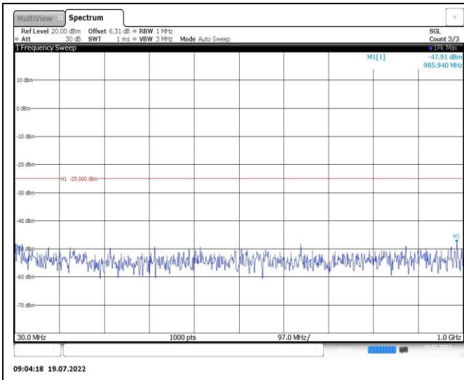
Band41-5MHz-QPSK-41565-1RB#0-Range1:30~1000MHz
