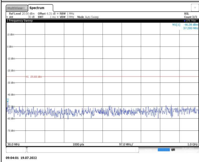
Band41-5MHz-16QAM-40620-1RB#0-Range1:30~1000MHz
