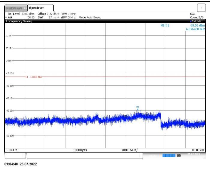
Band26-10MHz-16QAM-26740-1RB#0-Range2:1000~10000MHz
