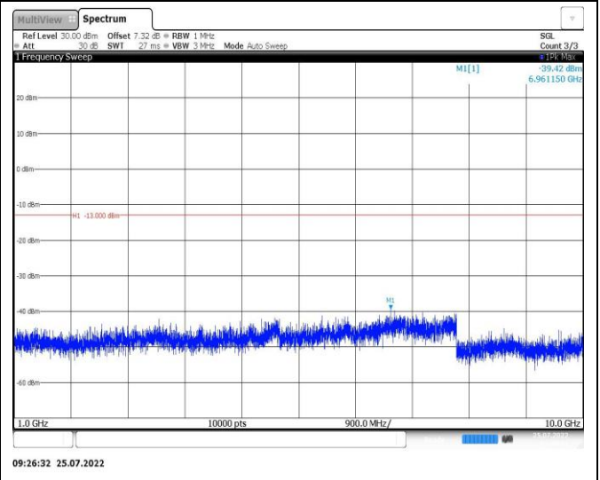
Band26-15MHz-16QAM-26865-1RB#0-Range2:1000~10000MHz
