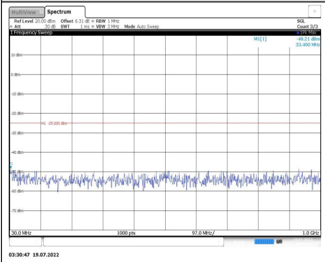
Band41-5MHz-QPSK-39675-1RB#0-Range1:30~1000MHz
