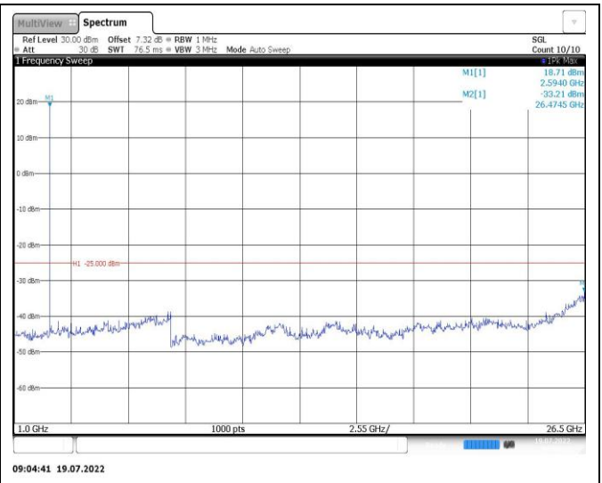
Band41-5MHz-16QAM-41565-1RB#0-Range2:1000~26500MHz
