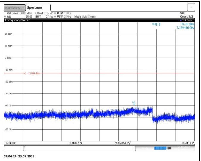
Band26-10MHz-16QAM-26990-1RB#0-Range2:1000~10000MHz
