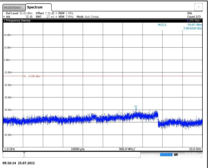
Band26-15MHz-16QAM-26965-1RB#0-Range2:1000~10000MHz
