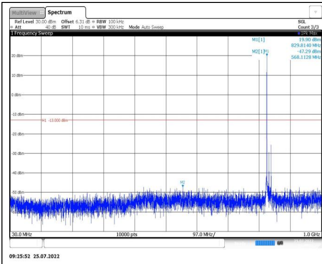
Band26-15MHz-QPSK-26965-1RB#0-Range1:30~1000MHz
