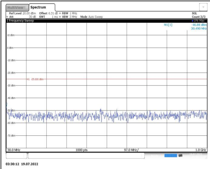
Band38-20MHz-16QAM-38150-1RB#0-Range1:30~1000MHz
