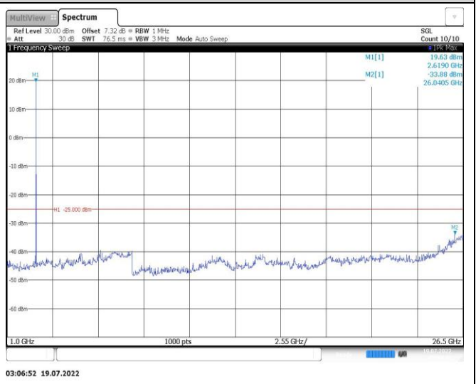
Band38-15MHz-QPSK-37825-1RB#0-Range2:1000~26500MHz
