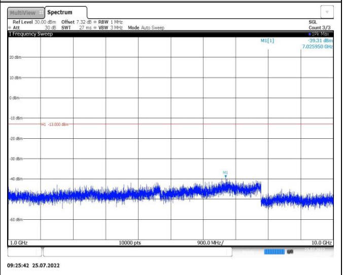
Band26-15MHz-16QAM-26915-1RB#0-Range2:1000~10000MHz
