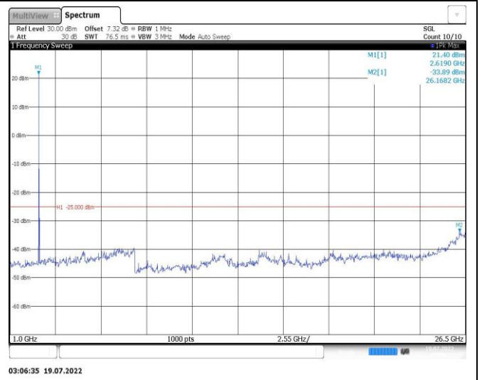
Band38-10MHz-16QAM-37800-1RB#0-Range2:1000~26500MHz
