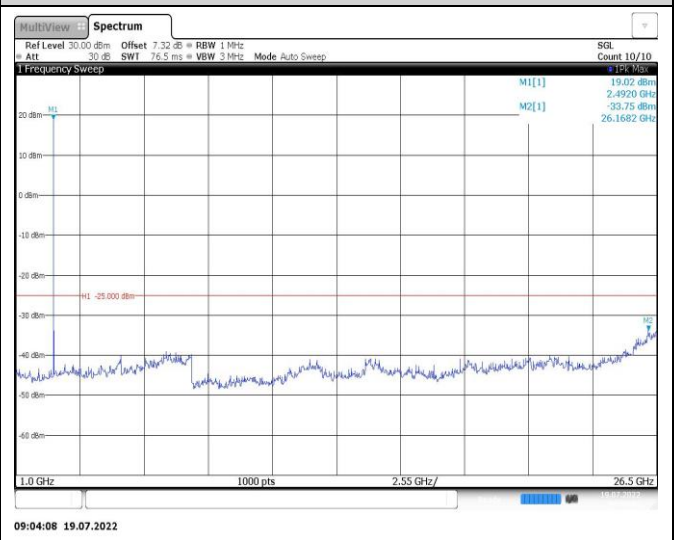
Band41-5MHz-16QAM-40620-1RB#0-Range2:1000~26500MHz
