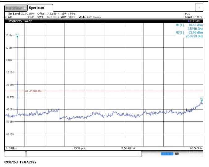
Band41-10MHz-16QAM-41540-1RB#0-Range2:1000~26500MHz
