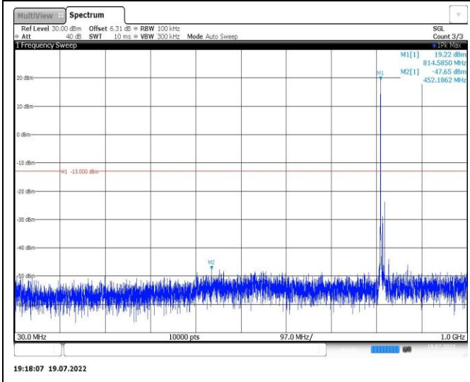
Band26-10MHz-16QAM-26840-1RB#0-Range1:30~1000MHz
