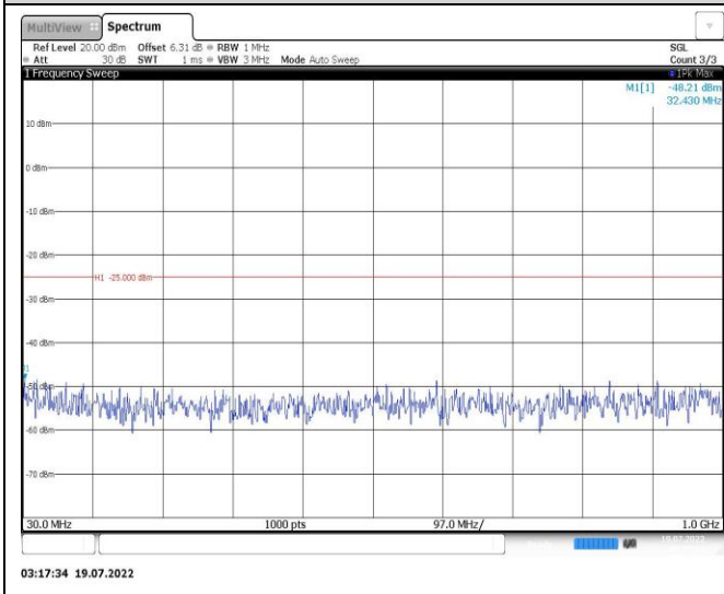
Band38-15MHz-16QAM-38000-1RB#0-Range1:30~1000MHz
