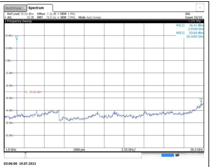
Band38-10MHz-QPSK-38200-1RB#0-Range2:1000~26500MHz
