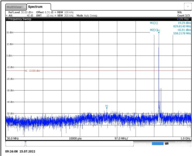
Band26-15MHz-16QAM-26965-1RB#0-Range1:30~1000MHz
