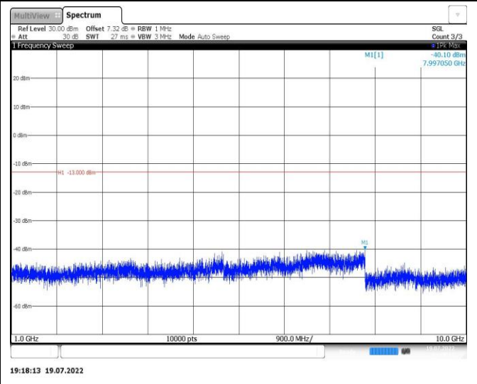
Band26-10MHz-16QAM-26840-1RB#0-Range2:1000~10000MHz
