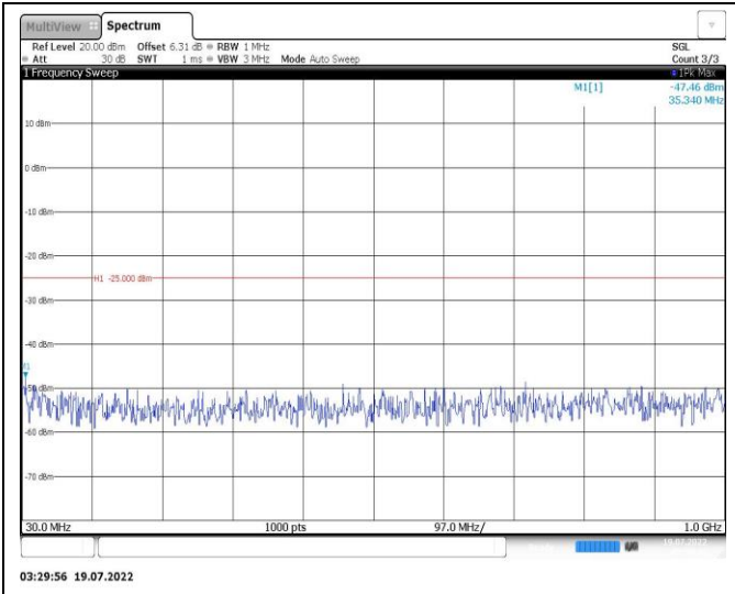
Band38-20MHz-QPSK-38150-1RB#0-Range1:30~1000MHz
