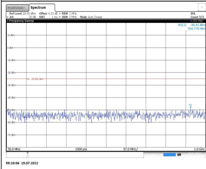
Band41-15MHz-QPSK-40620-1RB#0-Range1:30~1000MHz
