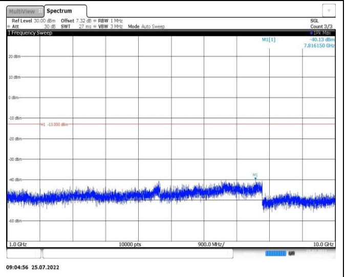
Band26-15MHz-QPSK-26865-1RB#0-Range2:1000~10000MHz
