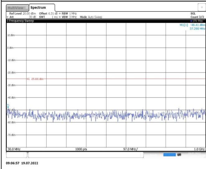
Band41-10MHz-QPSK-40620-1RB#0-Range1:30~1000MHz
