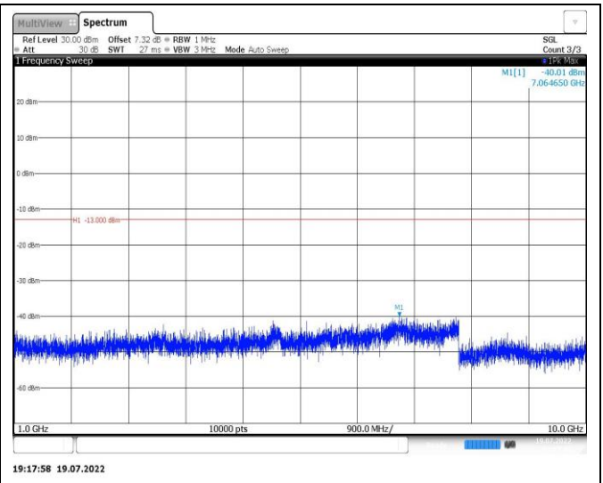
Band26-10MHz-QPSK-26840-1RB#0-Range2:1000~10000MHz
