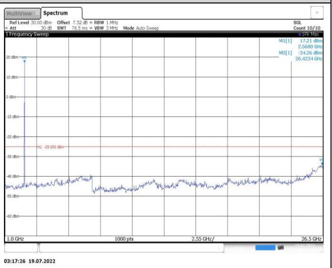
Band38-15MHz-QPSK-38000-1RB#0-Range2:1000~26500MHz
