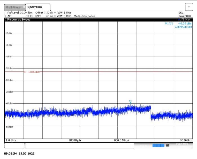
Band26-10MHz-16QAM-26915-1RB#0-Range2:1000~10000MHz
