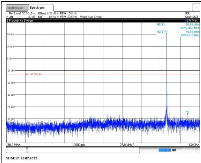
Band26-10MHz-16QAM-26990-1RB#0-Range1:30~1000MHz
