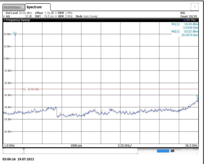
Band38-10MHz-16QAM-38200-1RB#0-Range2:1000~26500MHz
