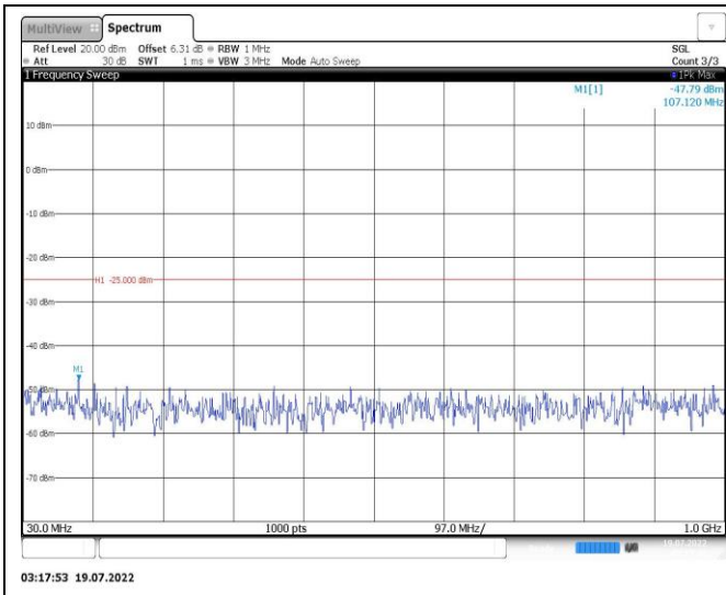
Band38-15MHz-QPSK-38175-1RB#0-Range1:30~1000MHz
