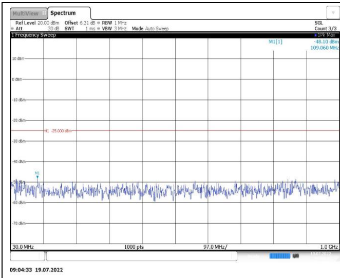
Band41-5MHz-16QAM-41565-1RB#0-Range1:30~1000MHz
