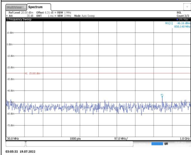
Band38-10MHz-16QAM-38000-1RB#0-Range1:30~1000MHz
