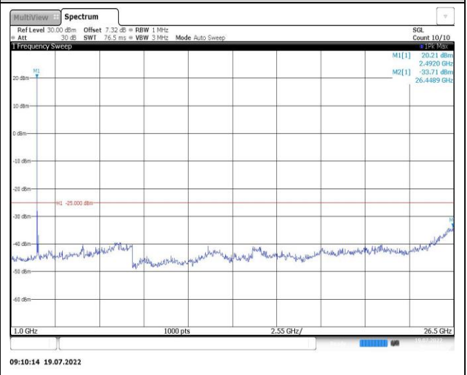
Band41-15MHz-QPSK-40620-1RB#0-Range2:1000~26500MHz
