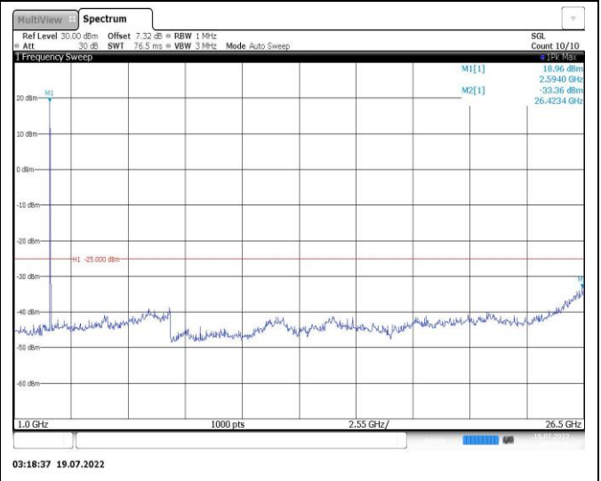
Band38-15MHz-16QAM-37825-1RB#0-Range2:1000~26500MHz
