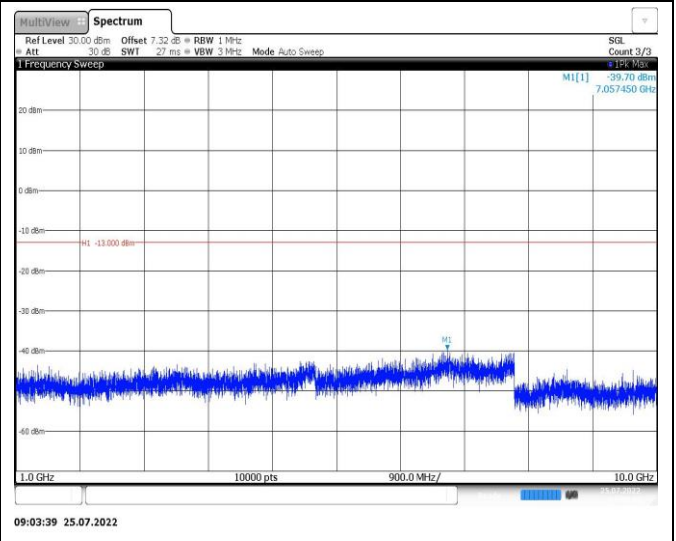
Band26-10MHz-QPSK-26915-1RB#0-Range2:1000~10000MHz
