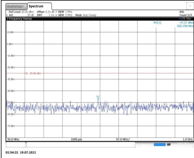
Band38-5MHz-16QAM-37775-1RB#0-Range1:30~1000MHz
