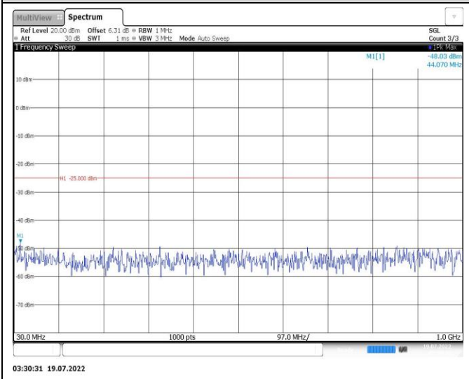
Band38-20MHz-16QAM-37850-1RB#0-Range1:30~1000MHz
