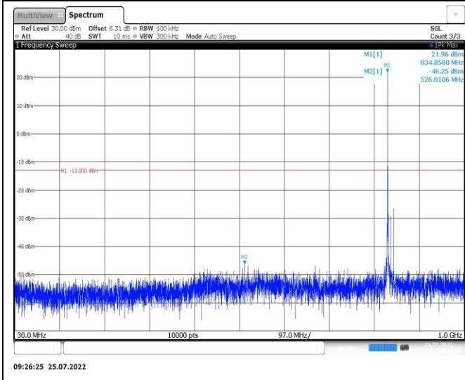
Band26-15MHz-16QAM-26865-1RB#0-Range1:30~1000MHz
