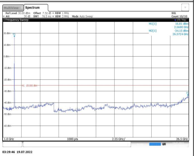
Band38-20MHz-16QAM-38000-1RB#0-Range2:1000~26500MHz
