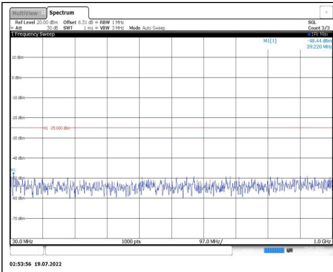
Band38-5MHz-QPSK-38225-1RB#0-Range1:30~1000MHz
