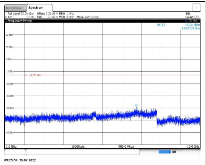
Band26-15MHz-QPSK-26965-1RB#0-Range2:1000~10000MHz
