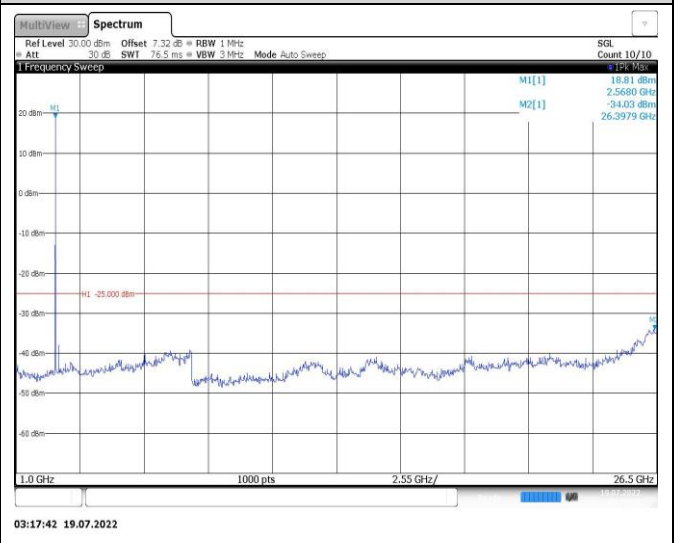
Band38-15MHz-16QAM-38000-1RB#0-Range2:1000~26500MHz
