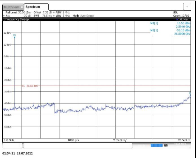
Band38-5MHz-16QAM-38225-1RB#0-Range2:1000~26500MHz
