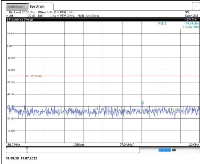
Band41-15MHz-QPSK-39725-1RB#0-Range1:30~1000MHz
