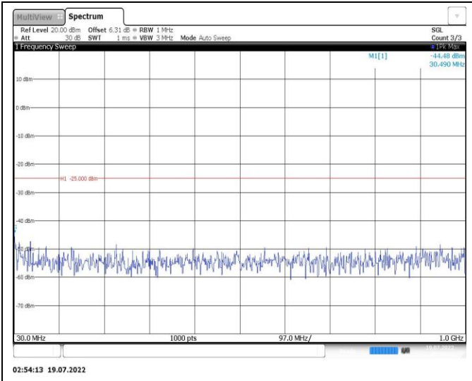
Band38-5MHz-16QAM-38225-1RB#0-Range1:30~1000MHz
