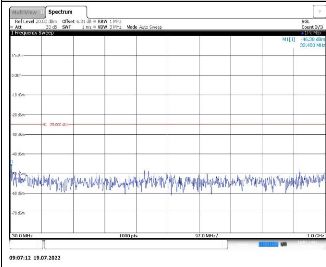
Band41-10MHz-16QAM-40620-1RB#0-Range1:30~1000MHz
