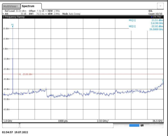
Band38-10MHz-QPSK-37800-1RB#0-Range2:1000~26500MHz
