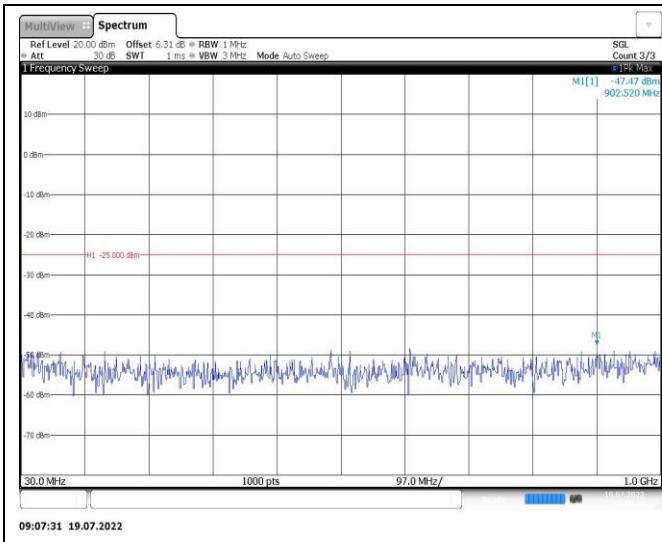
Band41-10MHz-QPSK-41540-1RB#0-Range1:30~1000MHz
