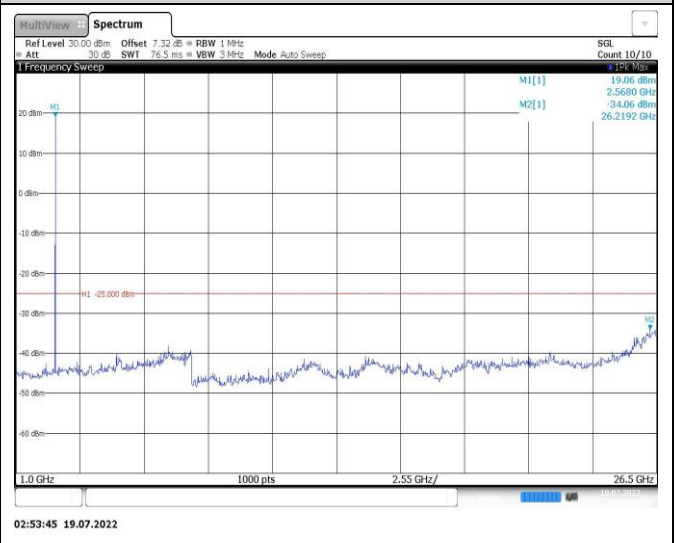
Band38-5MHz-16QAM-38000-1RB#0-Range2:1000~26500MHz
