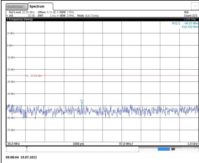
Band41-10MHz-16QAM-39700-1RB#0-Range1:30~1000MHz
