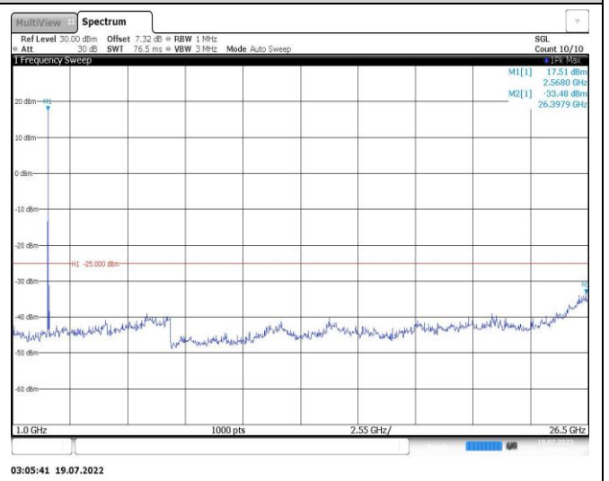
Band38-10MHz-16QAM-38000-1RB#0-Range2:1000~26500MHz
