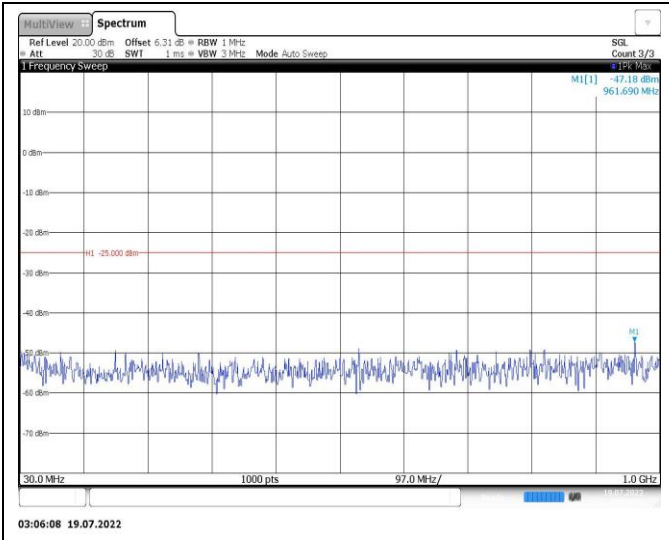
Band38-10MHz-16QAM-38200-1RB#0-Range1:30~1000MHz
