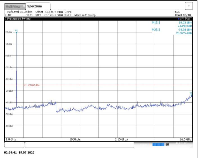
Band38-5MHz-16QAM-37775-1RB#0-Range2:1000~26500MHz
