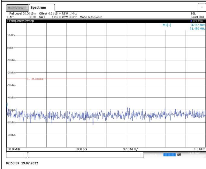
Band38-5MHz-16QAM-38000-1RB#0-Range1:30~1000MHz
