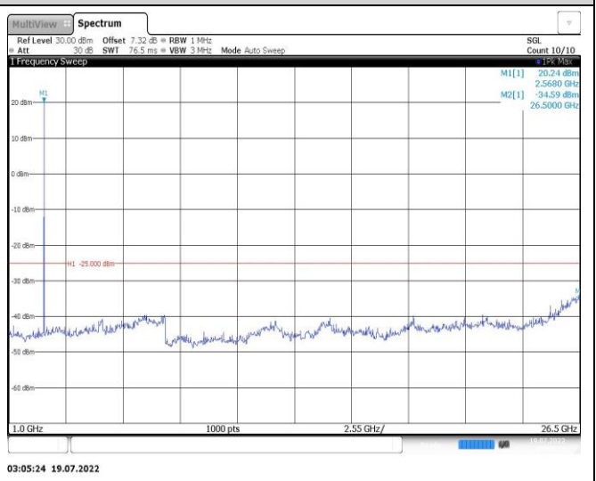
Band38-10MHz-QPSK-38000-1RB#0-Range2:1000~26500MHz
